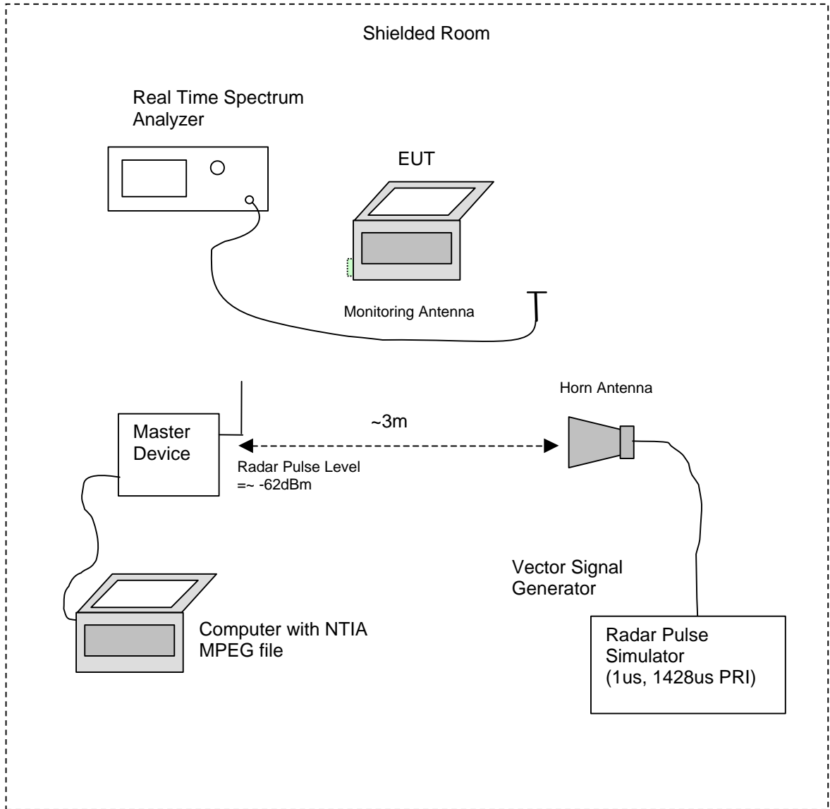
Figure 1: Radiated Test Setup for DFS
