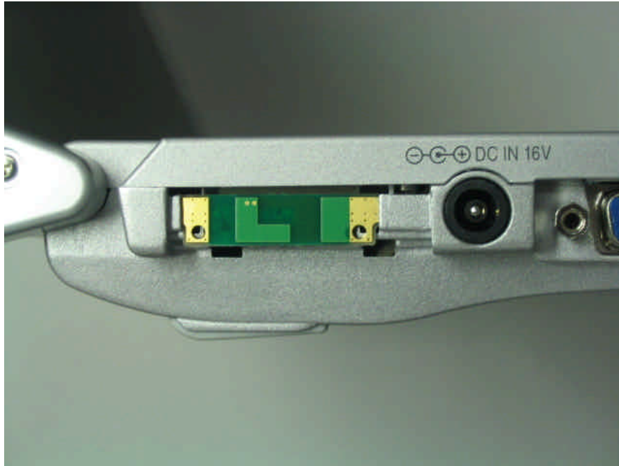
Aux TX/RX Antenna Magnified View
