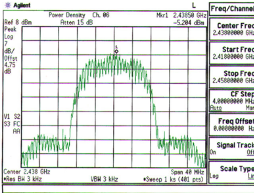
Plot A-8. FCC ID: ACJ9TGCF-W21 Max. Power Density Plot – Ch.6
