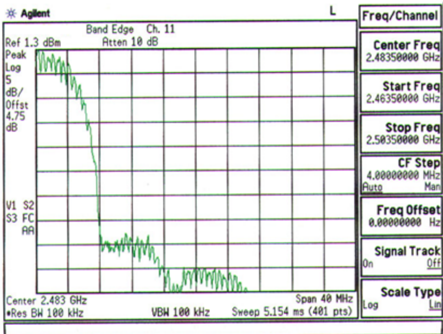
Plot A-12. FCC ID: ACJ9TGCF-W21 BandEdge Plot – Ch.11
