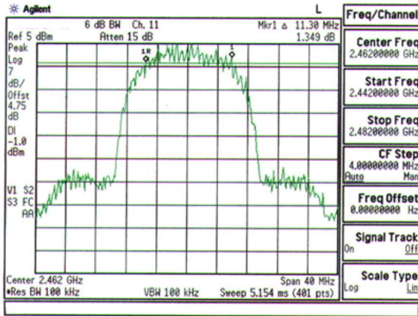
Plot A-3. FCC ID: ACJ9TGCF-W21 6dB Bandwidth Plot – Ch.11
