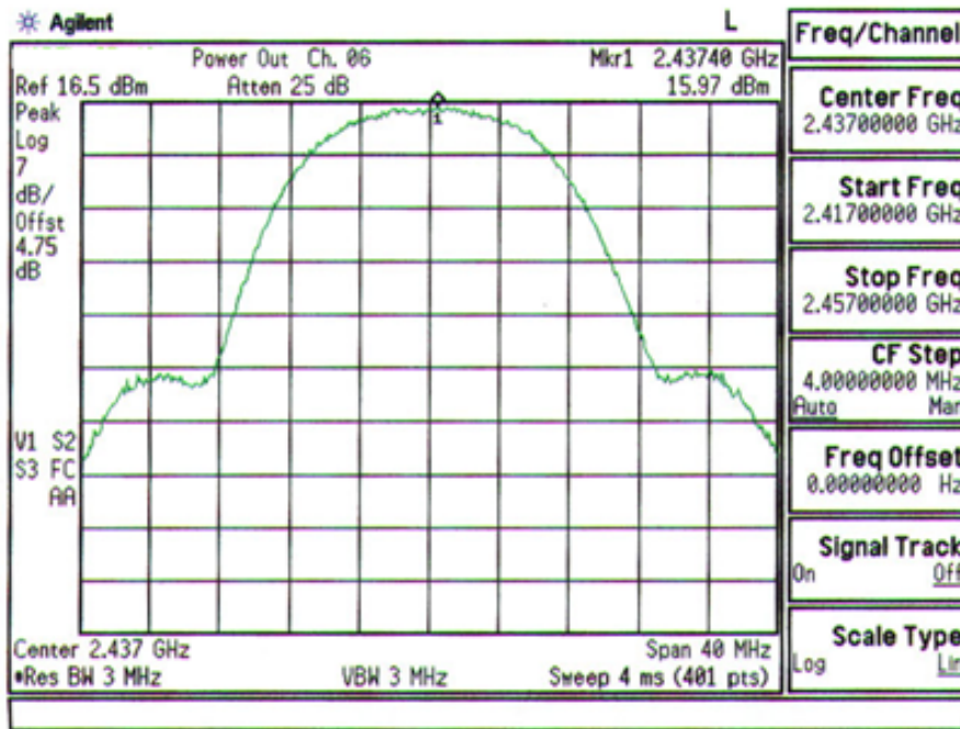
Plot A-5. FCC ID: ACJ9TGCF-W21 Max. Peak Output Power Plot – Ch.6
