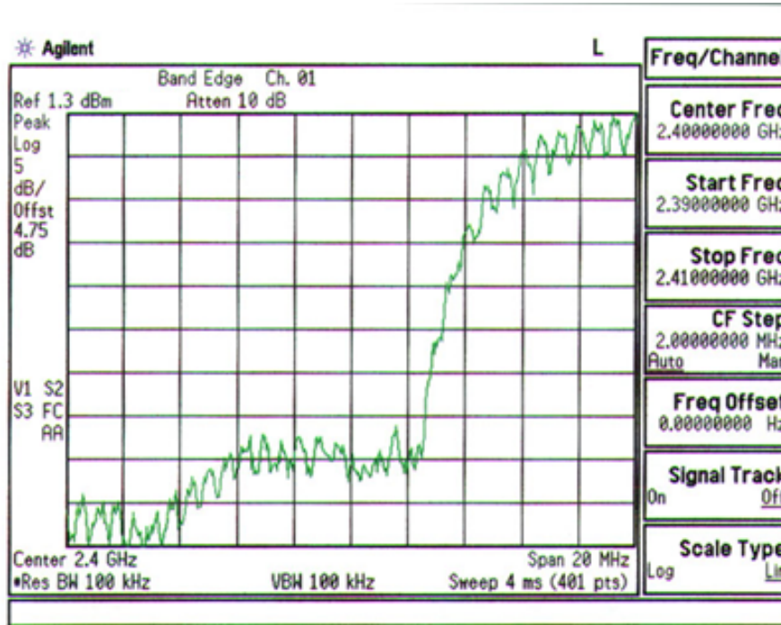
Plot A-10. FCC ID: ACJ9TGCF-W21 BandEdge Plot – Ch.1
