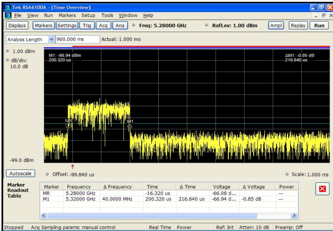
Figure 5-7. Pulse Width After 200ms
