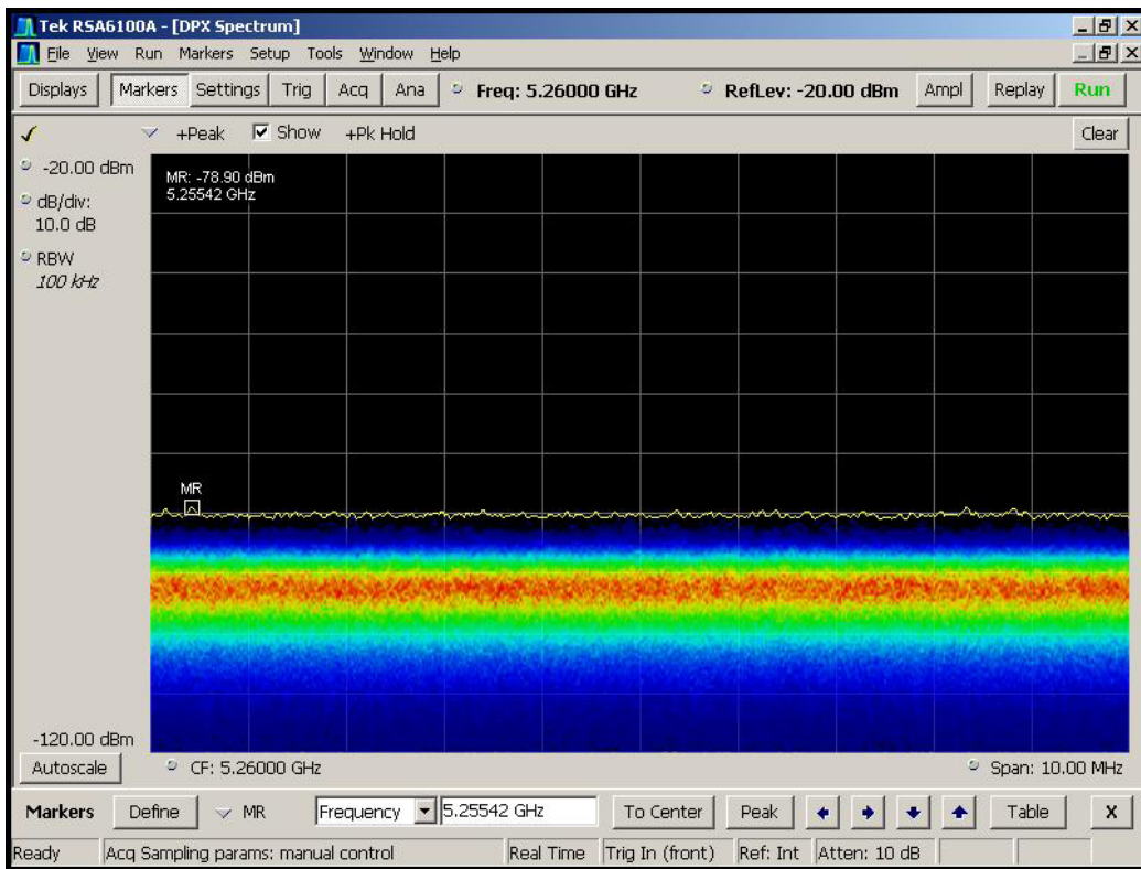
Figure 5-8 Non-occupancy Period - Monitoring live real time spectrum - Elapse time 30 minutes
