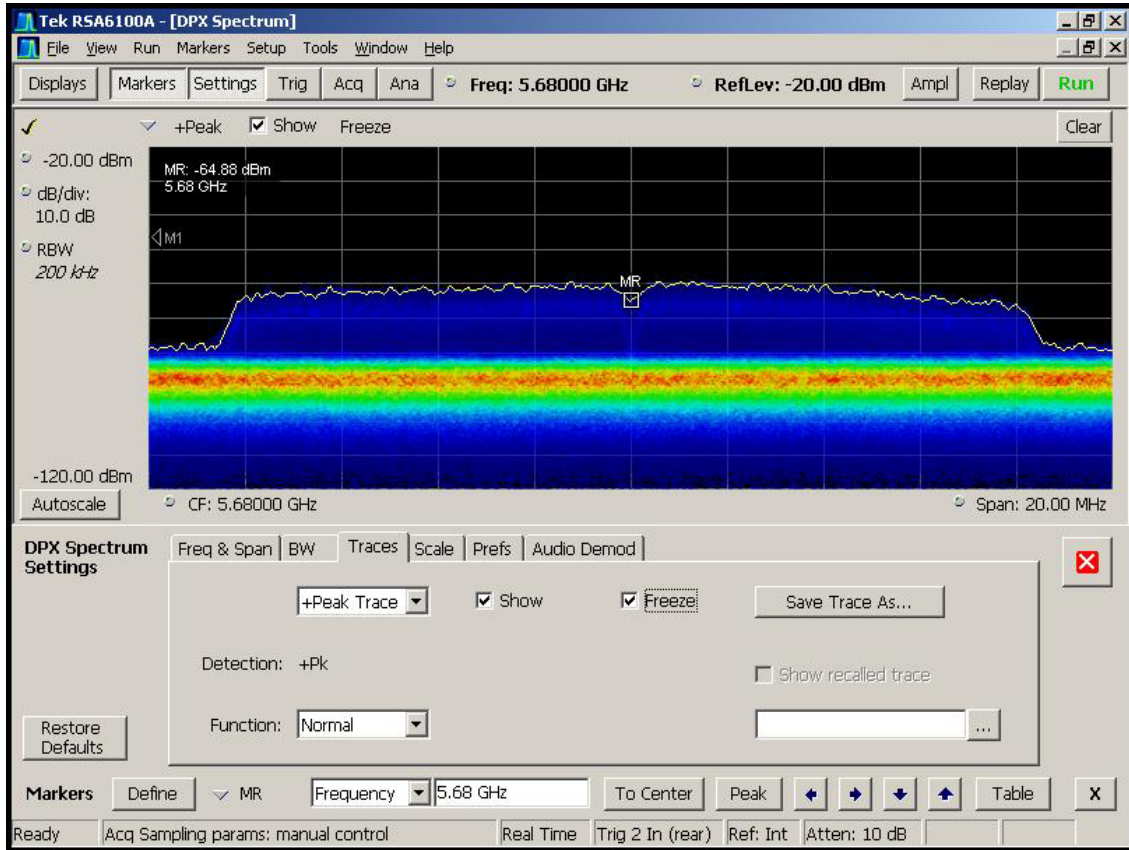
Figure 6-3. Real-Time Spectrum Display, WLAN Traffic (Streaming Video)
