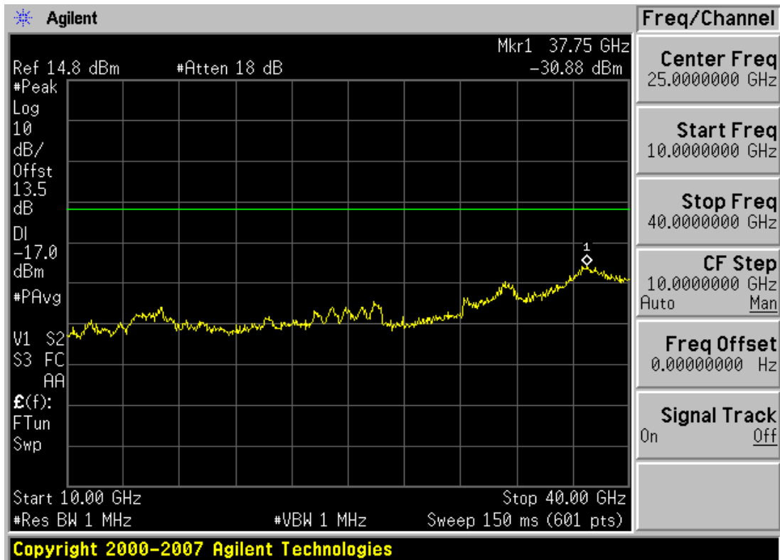
Plot 6-48. Conducted Spurious Plot (802.11a – Ch. 157)
