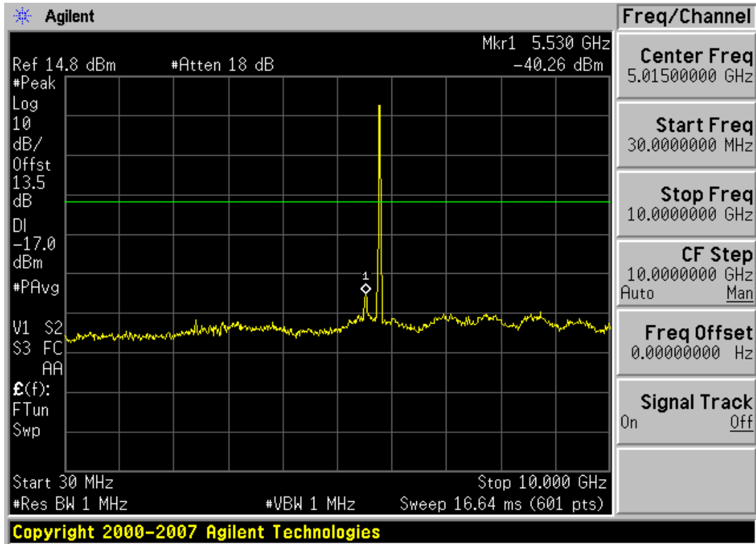
Plot 6-47. Conducted Spurious Plot (802.11a – Ch. 157)
