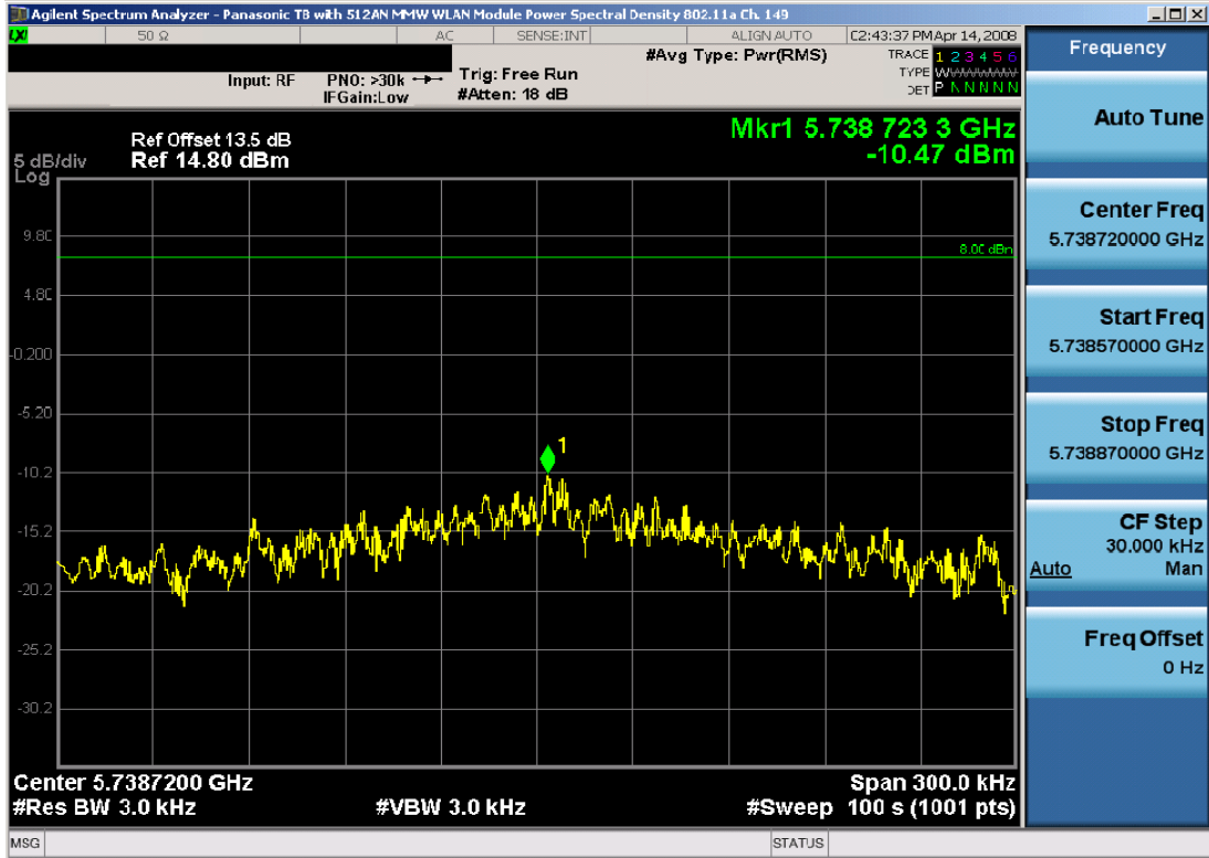
Plot 6-21. Power Spectral Density Plot (802.11a – Ch. 149)
