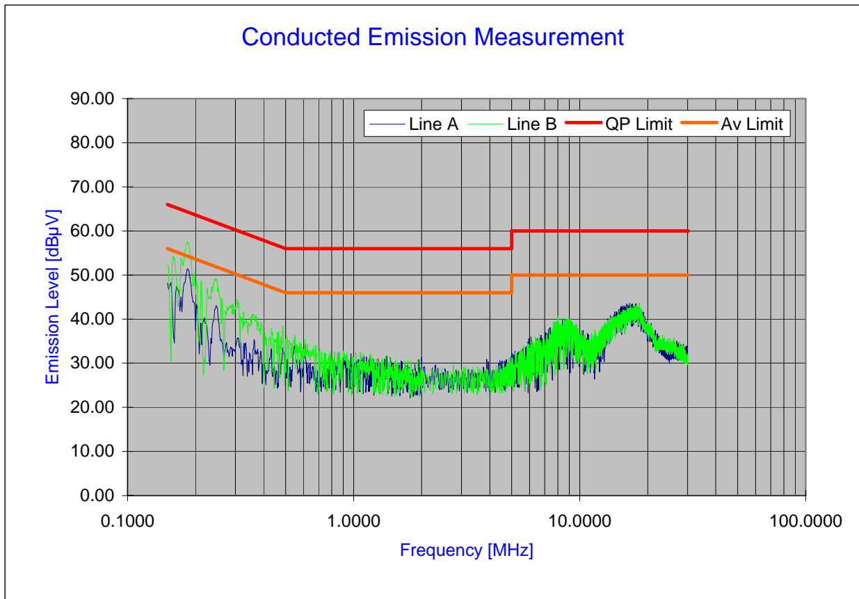
Plot 6-52. Line Conducted Plot with 802.11g
