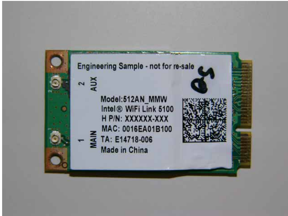
WLAN Exterior Top View
