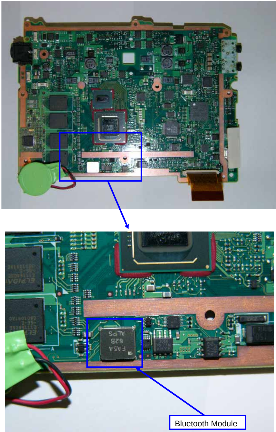
Bluetooth Top View on Main Board
