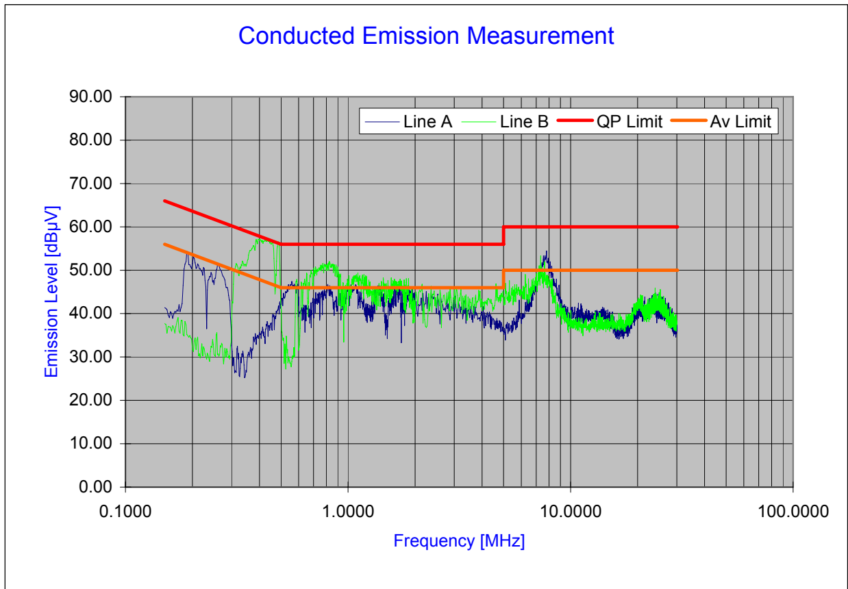
Plot 6-54. Line Conducted Plot with 802.11n (UNII Band III)
