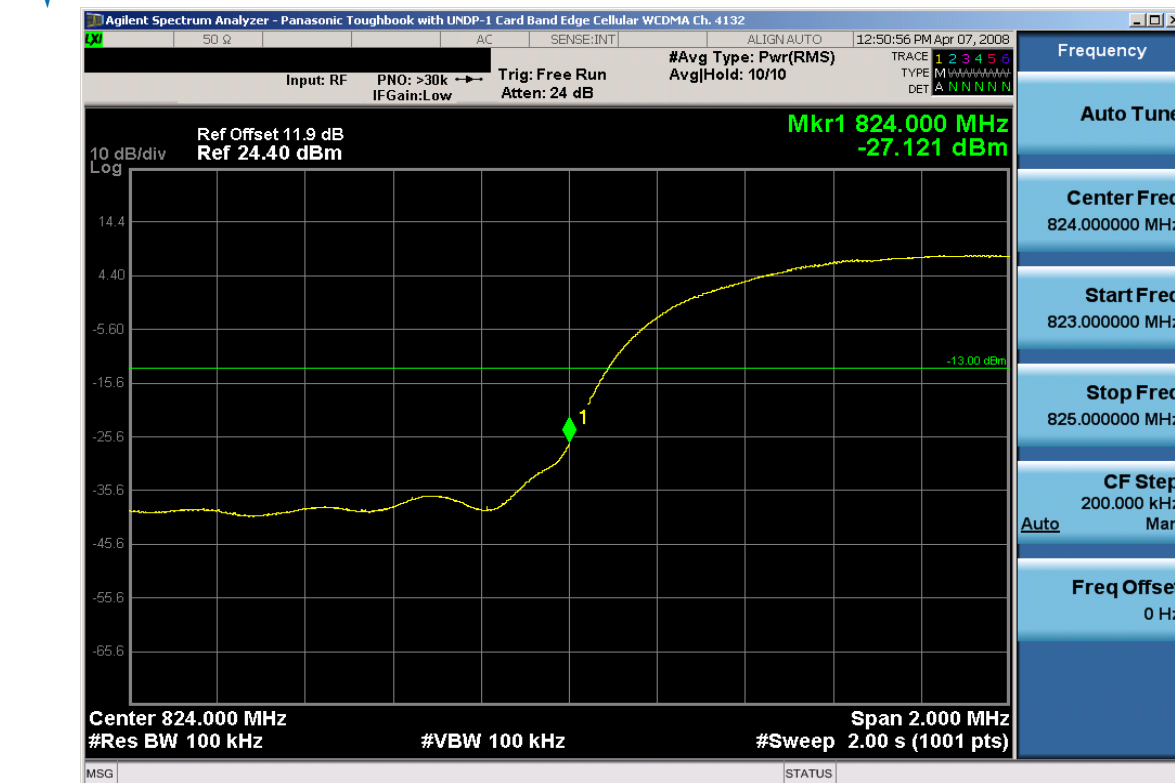
Plot 7-25. Band Edge Plot (Cellular WCDMA Mode – Ch. 4132)
