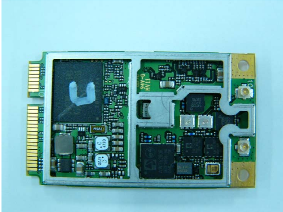
HSDPA3.6 Inside Top View
