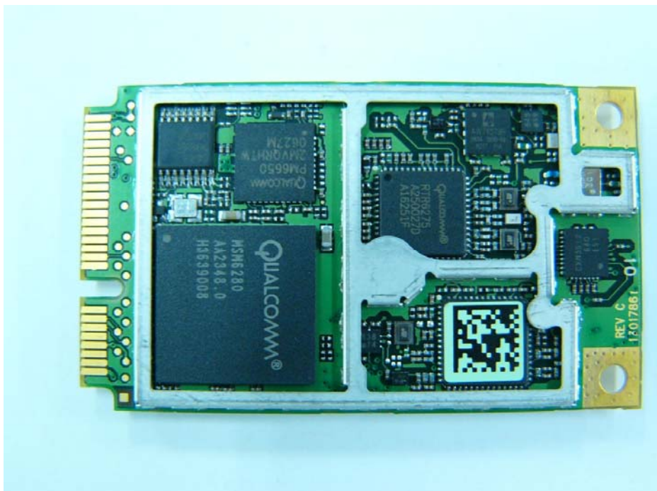
HSDPA3.6 Inside Bottom View
