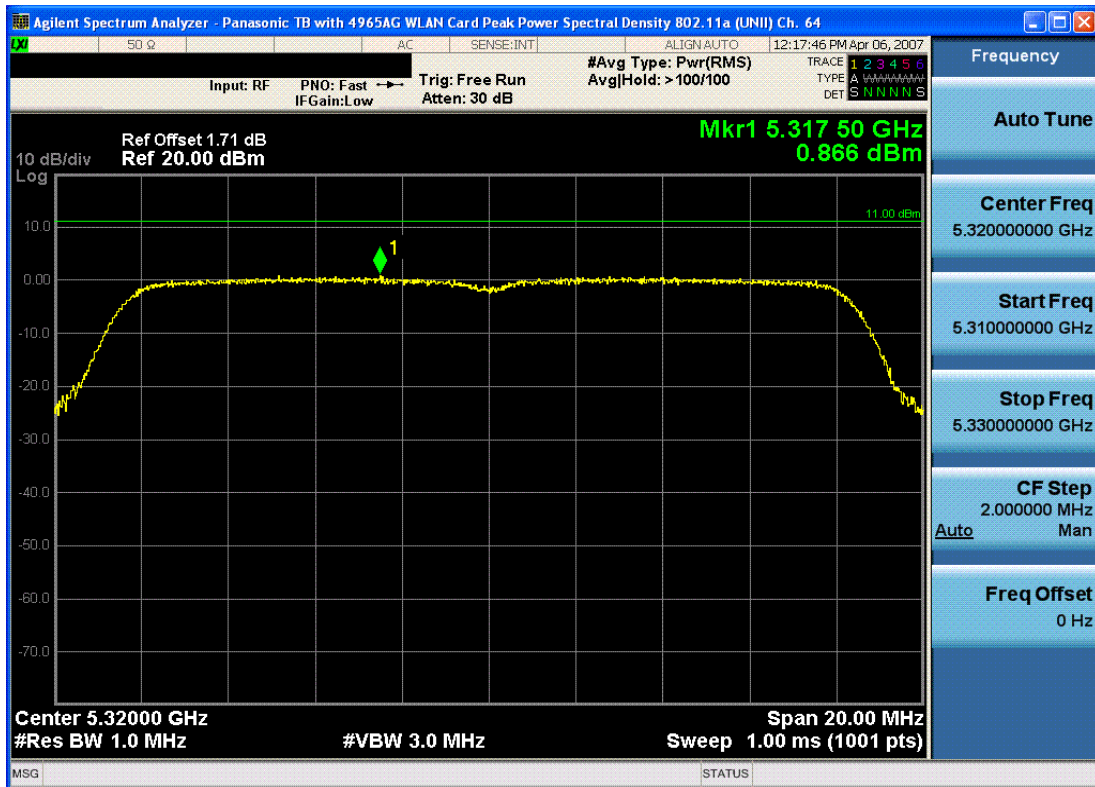
Plot 6-7. Peak Power Spectral Density Plot [FCC / IC] (802.11a (UNII) – Ch. 64)
