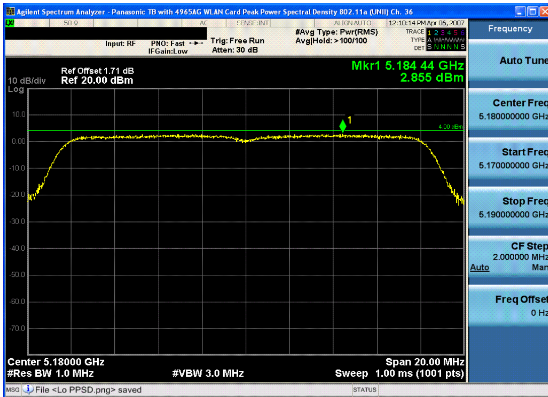
Plot 6-4. Peak Power Spectral Density Plot [FCC] (802.11a (UNII) – Ch. 36)
