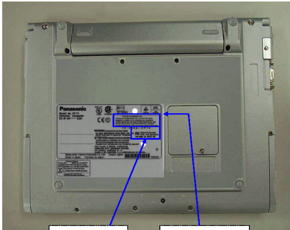
Rating Plate (FCC DoC Position)
