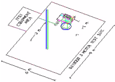
Figure 5. Turntable and System Setup
