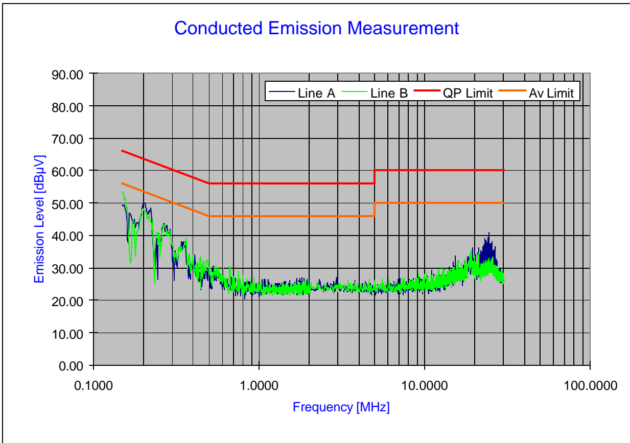
Plot 6-41. Line Conducted Plot with 802.11a (UNII Band II)
