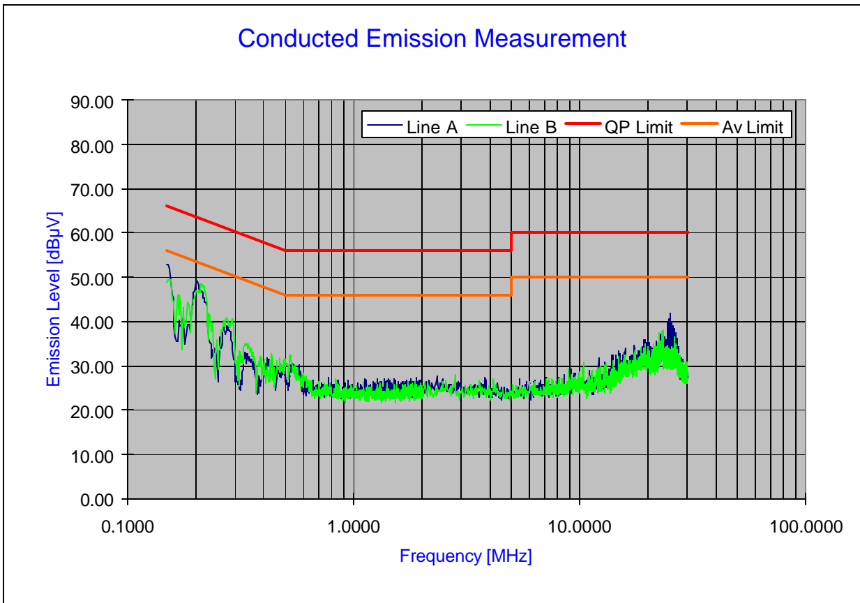
Plot 6-40. Line Conducted Plot with 802.11a (UNII Band I)
