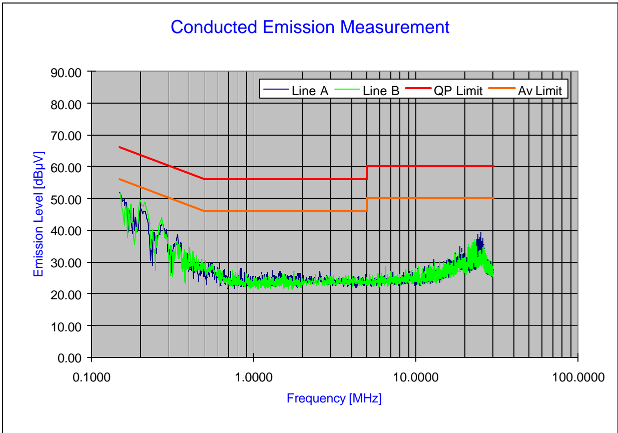
Plot 6-42. Line Conducted Plot with 802.11a (UNII Band III)
