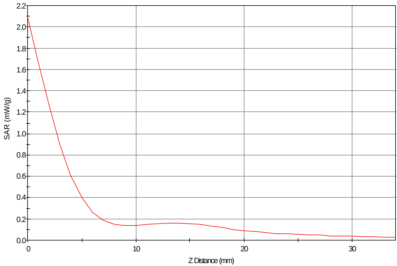
SAR - Z Axis at Hotspot x:18.0 y:70.0
