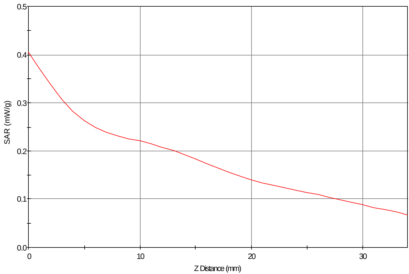
SAR - Z Axis at Hotspot x:26.0 y:14.0
