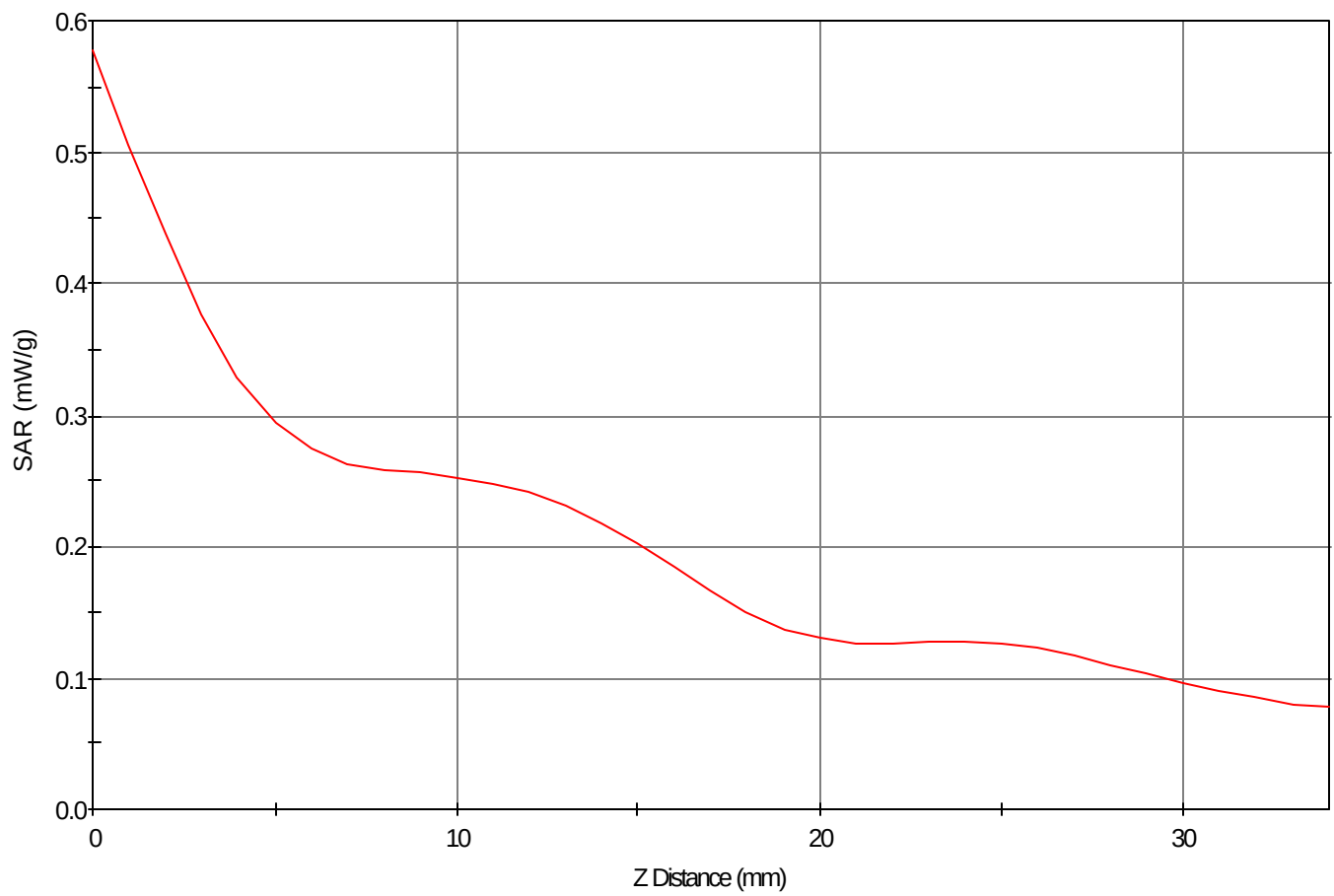
SAR - Z Axis at Hotspot x:32.0 y:-7.0
