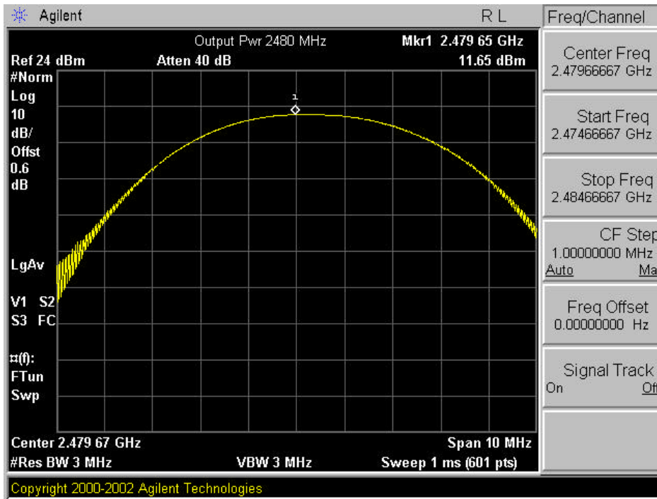
Plot A-6. Max. Peak Output Power Plot – Ch. 89
