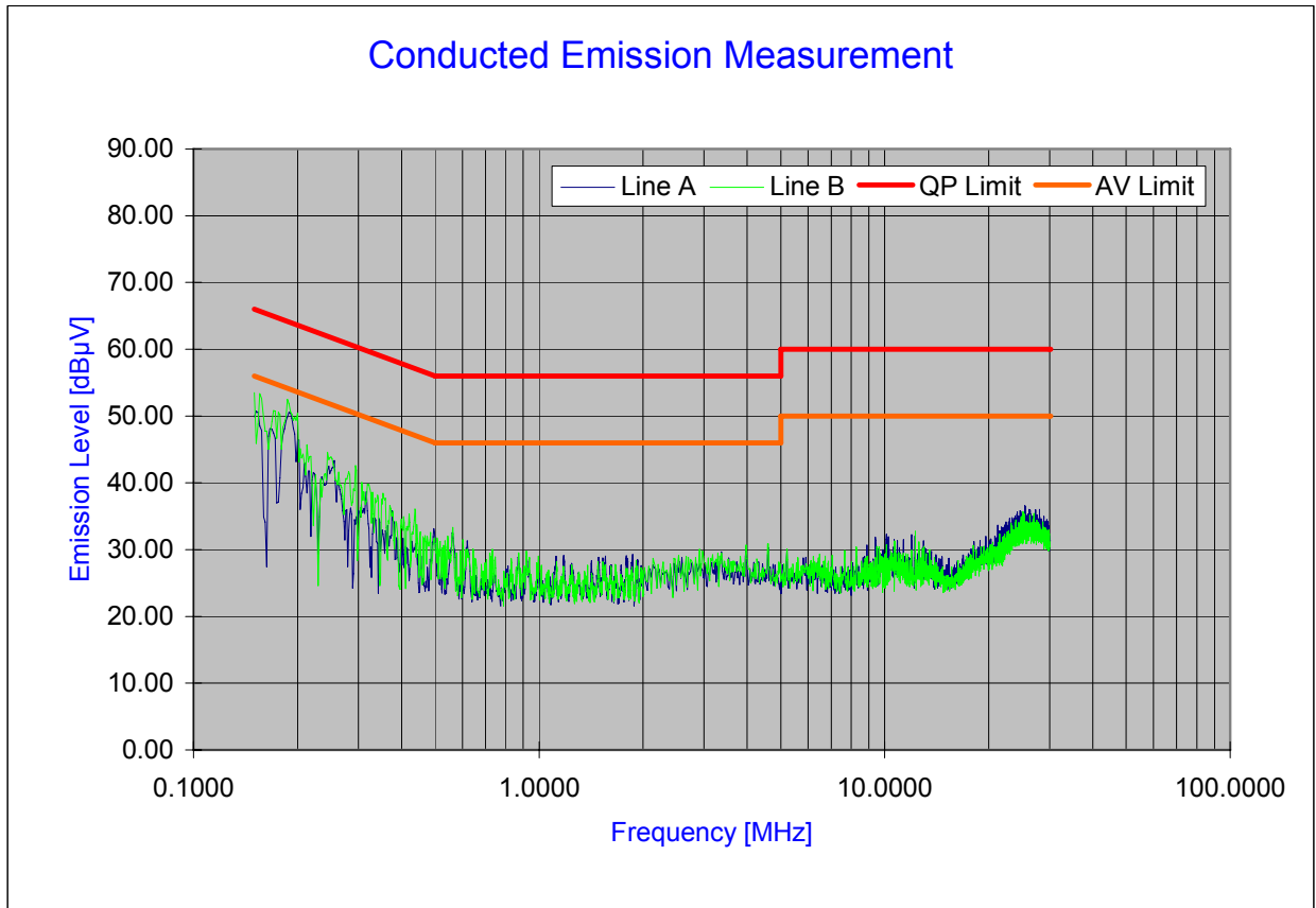
Plot 8-2. Line-Conducted Test Plot
