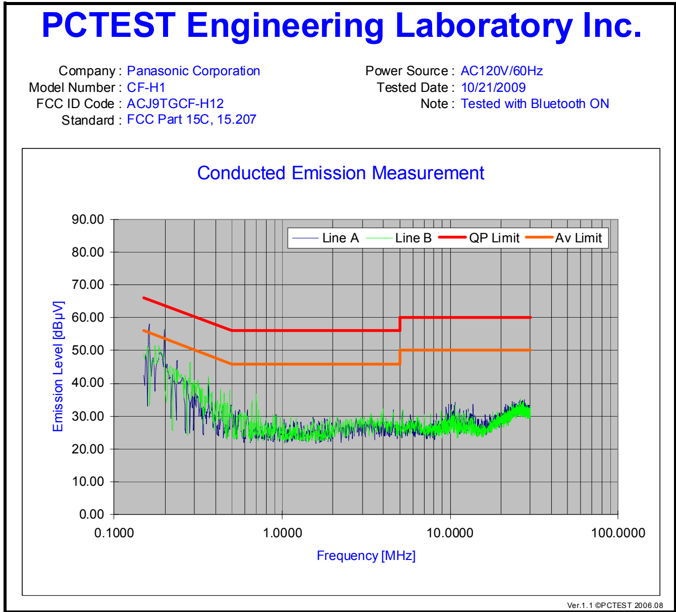
Plot 6-18. Line Conducted Plot with Bluetooth
