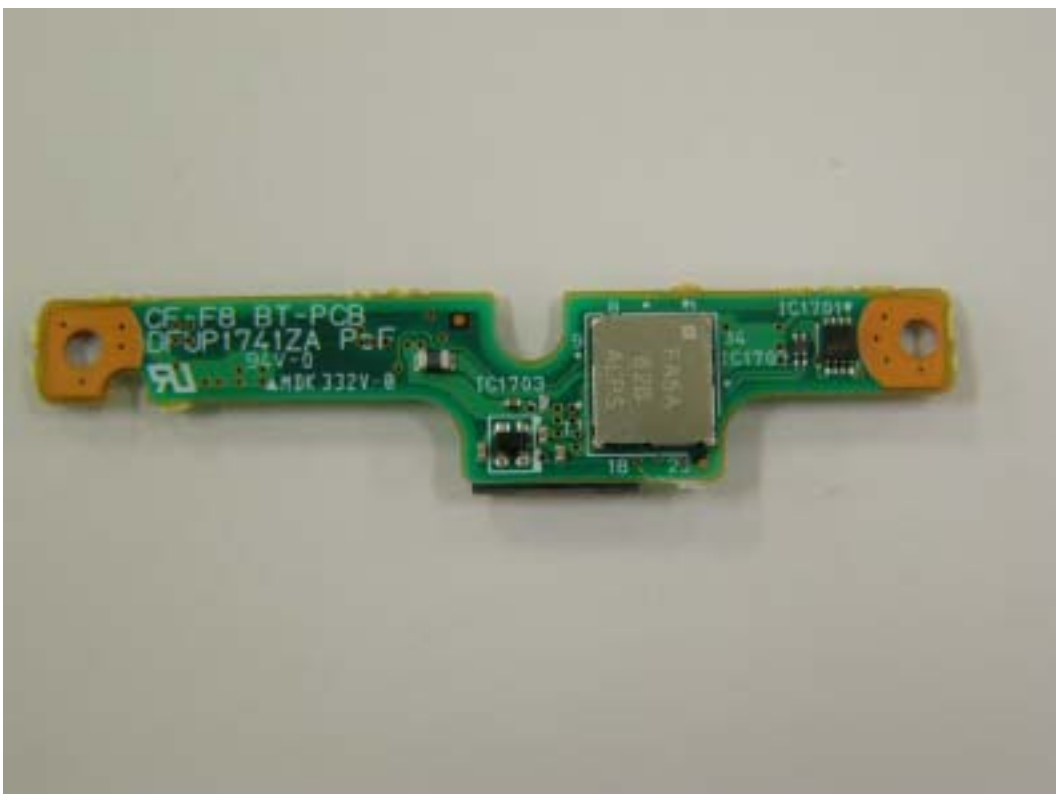
Bluetooth Card Bottom View
