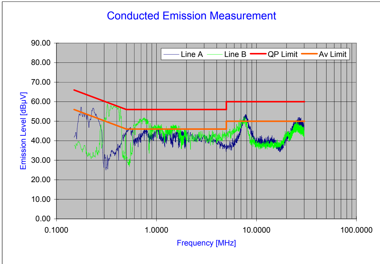
Plot 6-49. Line Conducted Plot with 802.11a (UNII Band I)
