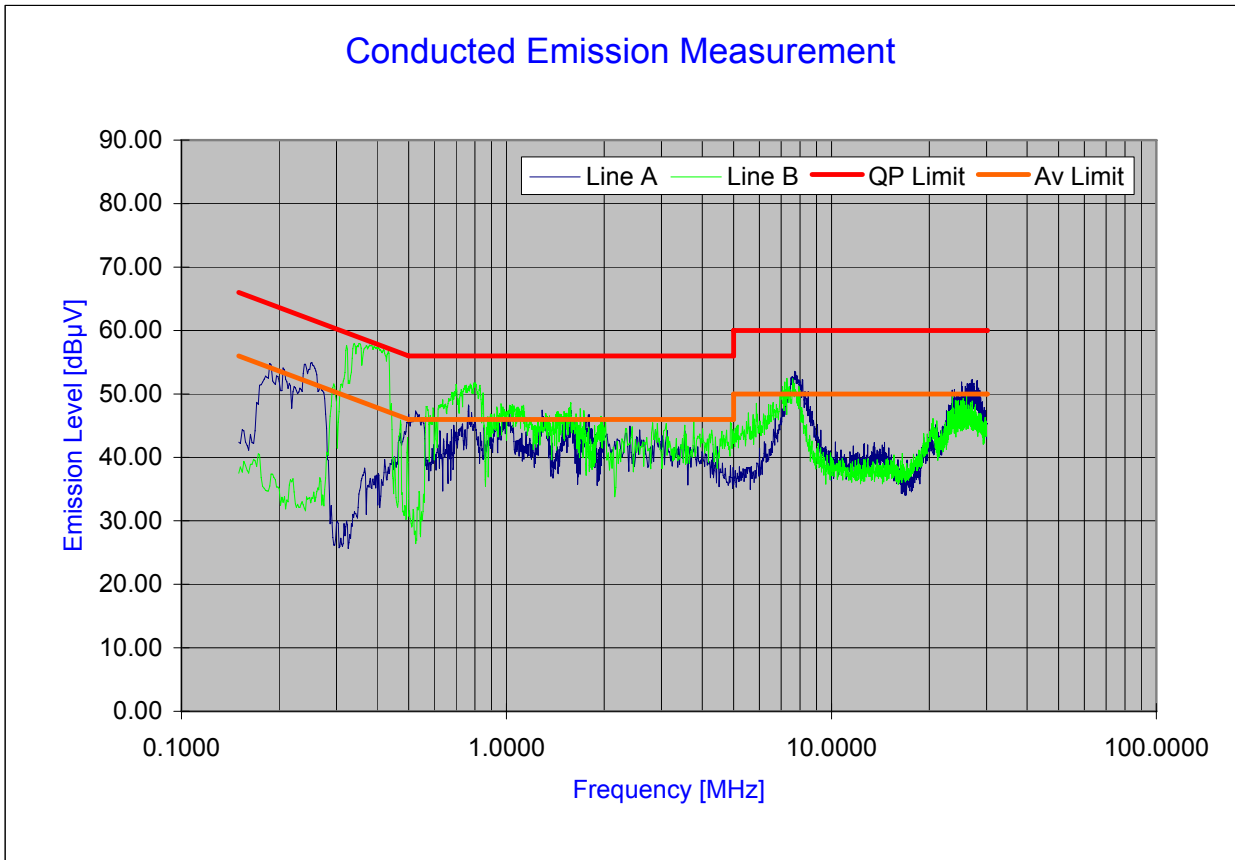
Plot 6-50. Line Conducted Plot with 802.11a (UNII Band II)
