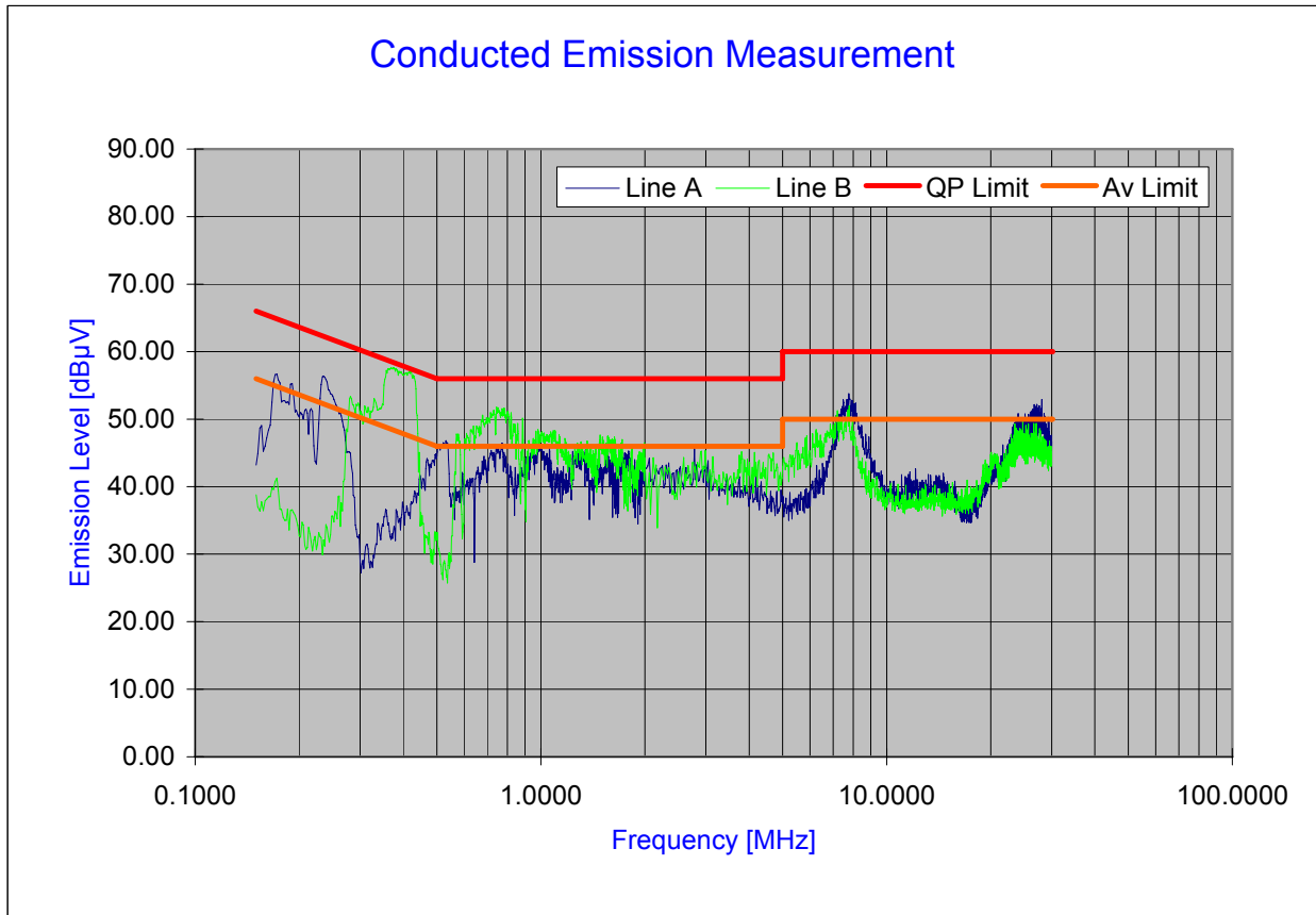
Plot 6-52. Line Conducted Plot with 802.11n (UNII Band I)
