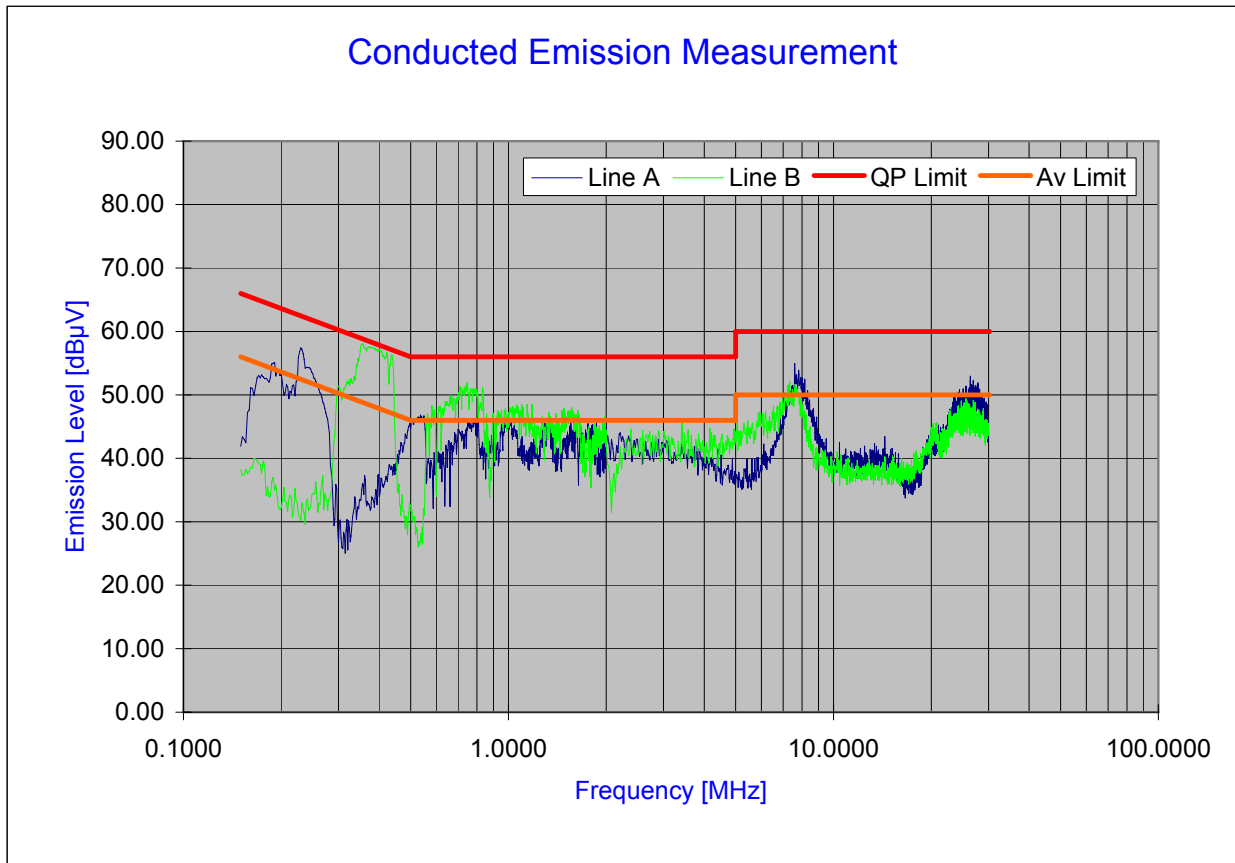
Plot 6-51. Line Conducted Plot with 802.11a (UNII Band III)
