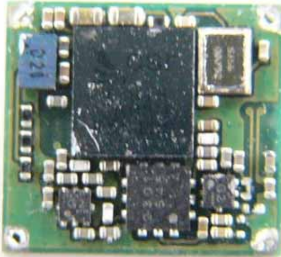
Bluetooth Module inside Top View
