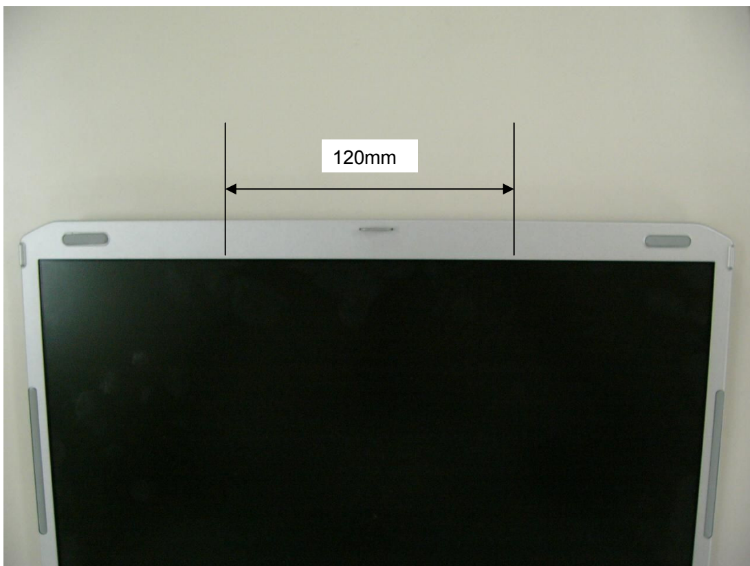
WWAN Aux RX Antenna
