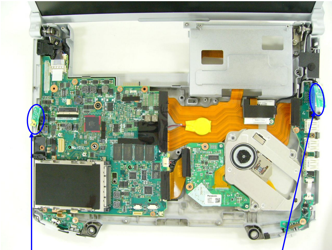
WLAN Aux RX Antenna
