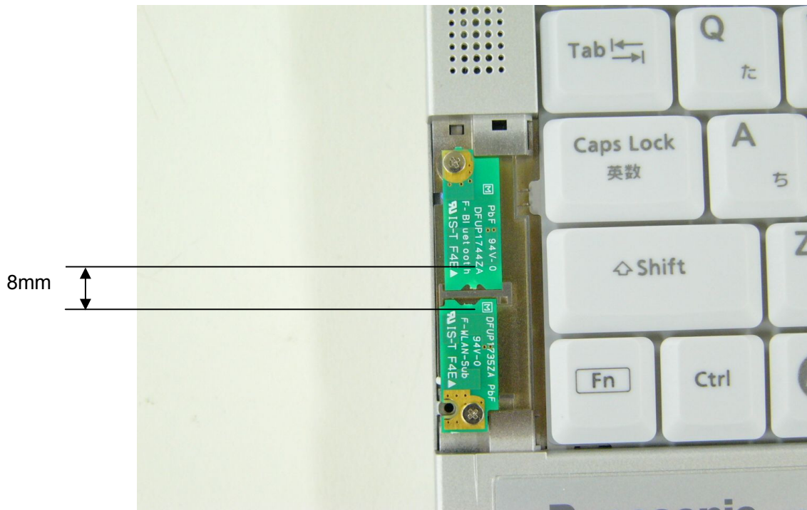
WLAN Aux RX Antenna
