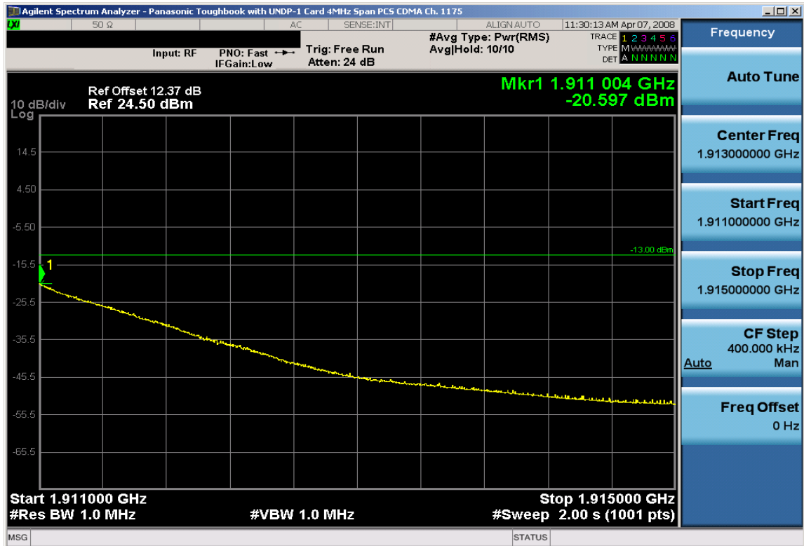
Plot 7-68. 4MHz Span Plot (PCS CDMA Mode – Ch. 1175)
