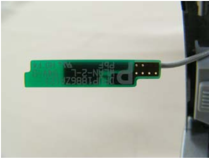
WLAN Aux TX/RX antenna magnified view (Top)
