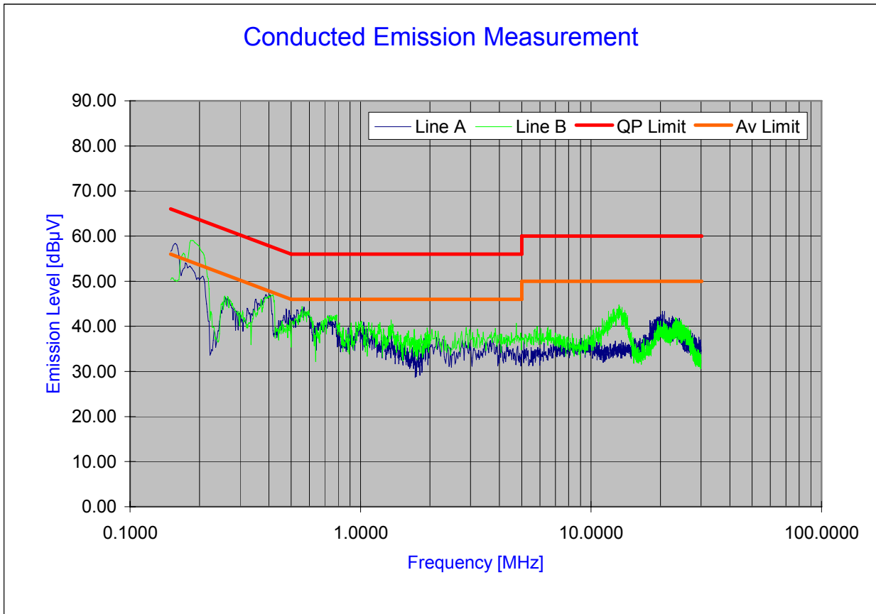
Plot 6-76. Line Conducted Plot with 802.11b
