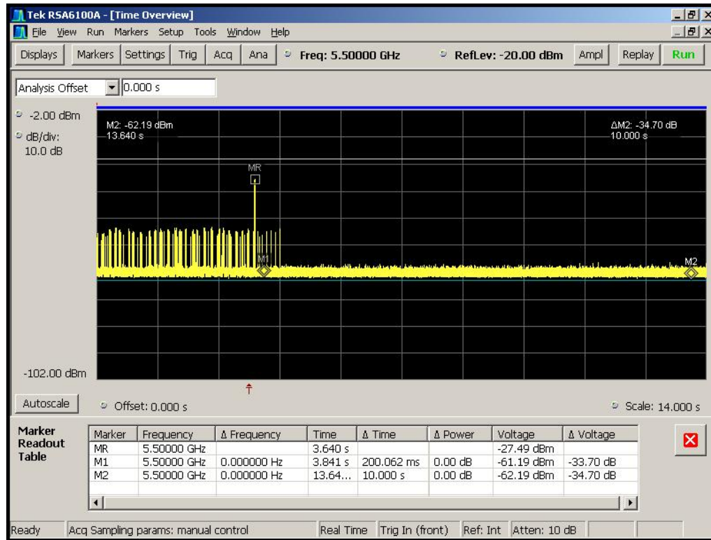
Figure 5-1. Channel Move Time (< 10sec)
