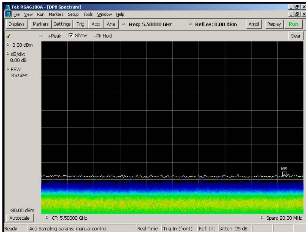
Figure 5-4 Non-occupancy Period – Monitoring live real time spectrum – elapsed time 30 minutes
