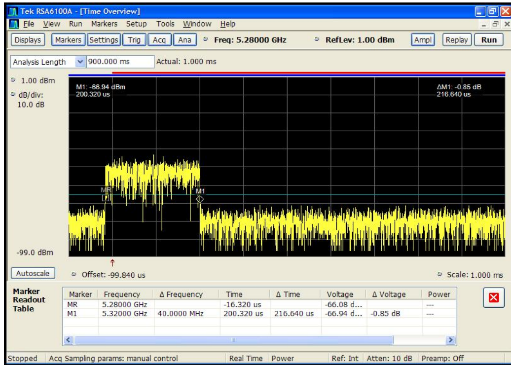
Figure 5-3. Pulse Width After 200ms
