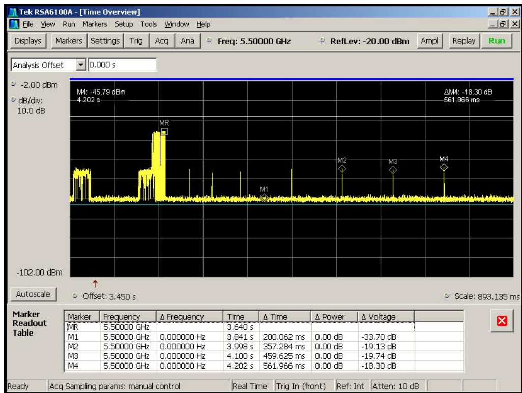
Figure 5-2. Channel Closing Transmission Time, Aggregate Time After 200ms
