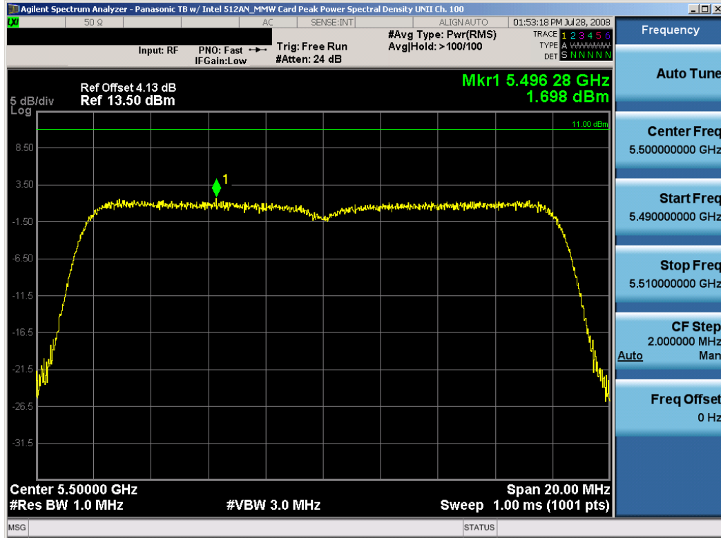
Plot 6-7. Peak Power Spectral Density Plot (802.11a (UNII) – Ch. 100)
