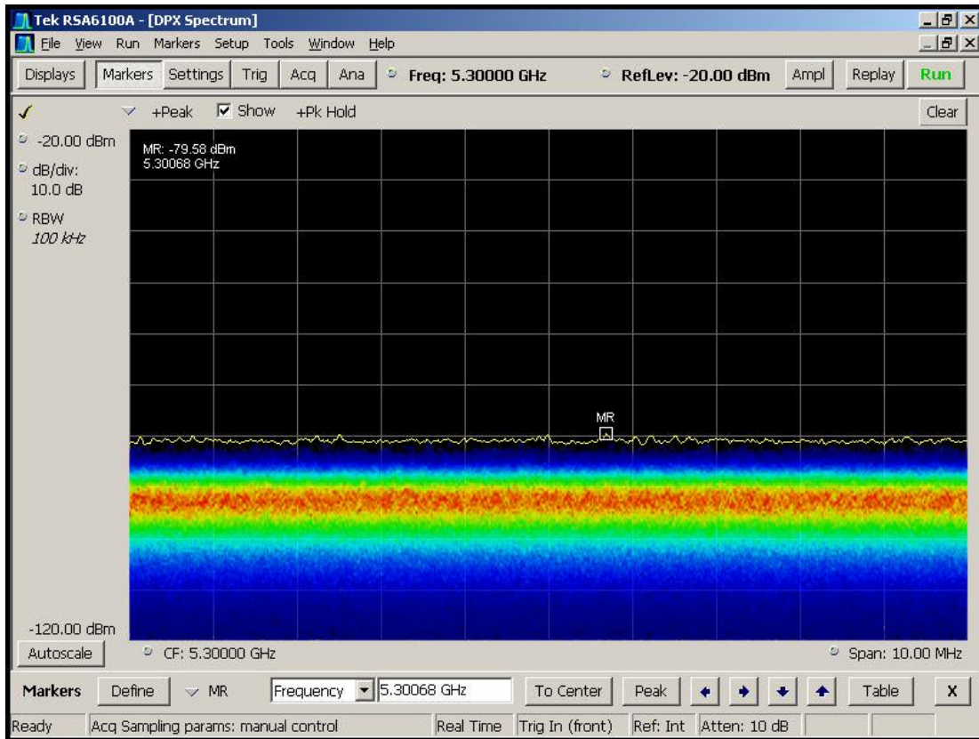
Figure 5-9 Non-occupancy Period After Startup - Monitoring live real time spectrum - Elapse time 30min
