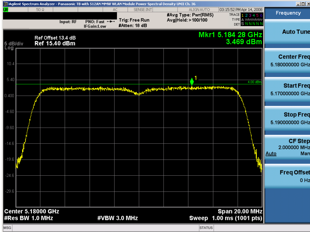
Plot 6-11. Peak Power Spectral Density Plot (802.11a (UNII) – Ch. 36)
