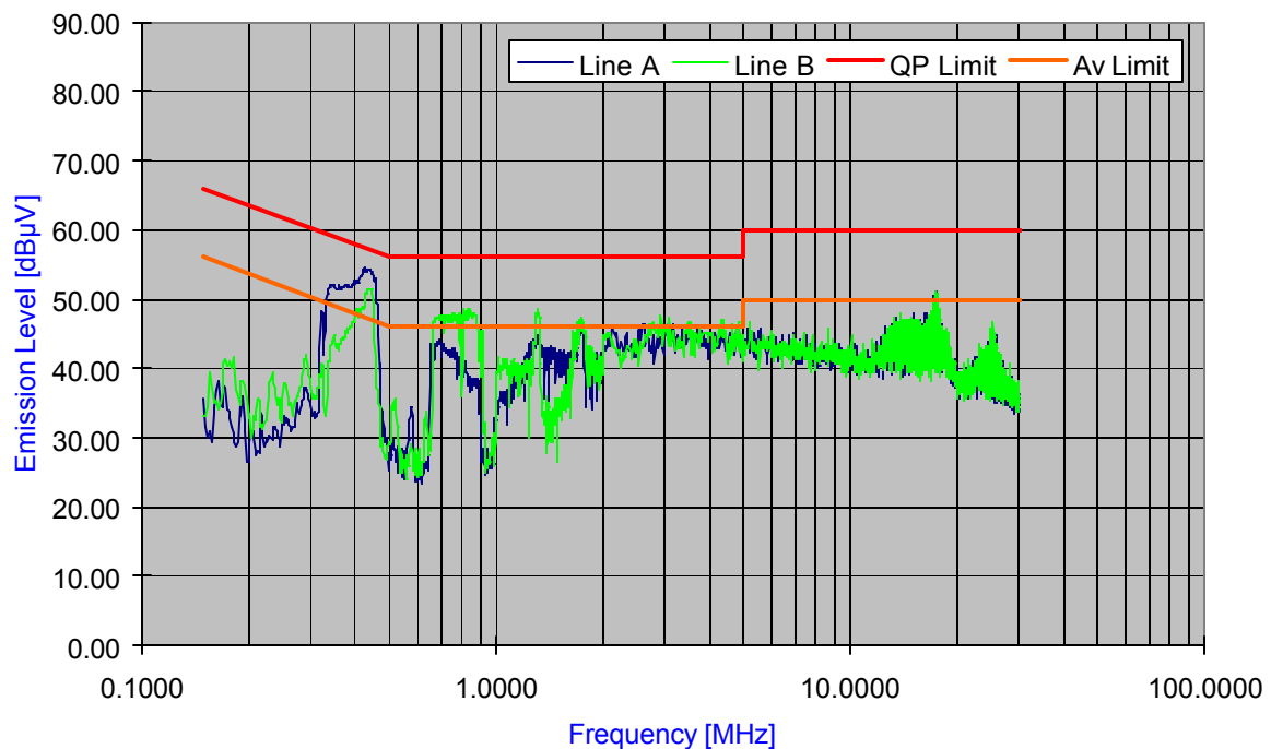
Plot 6-33. Line Conducted Plot with 802.11n (UNII-I Band)
