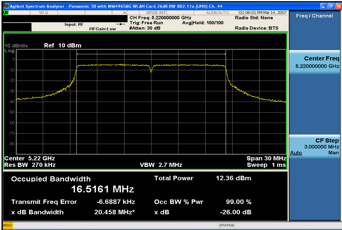
Plot 6-2. 26dB Bandwidth Plot (802.11a (UNII) – Ch. 44)
