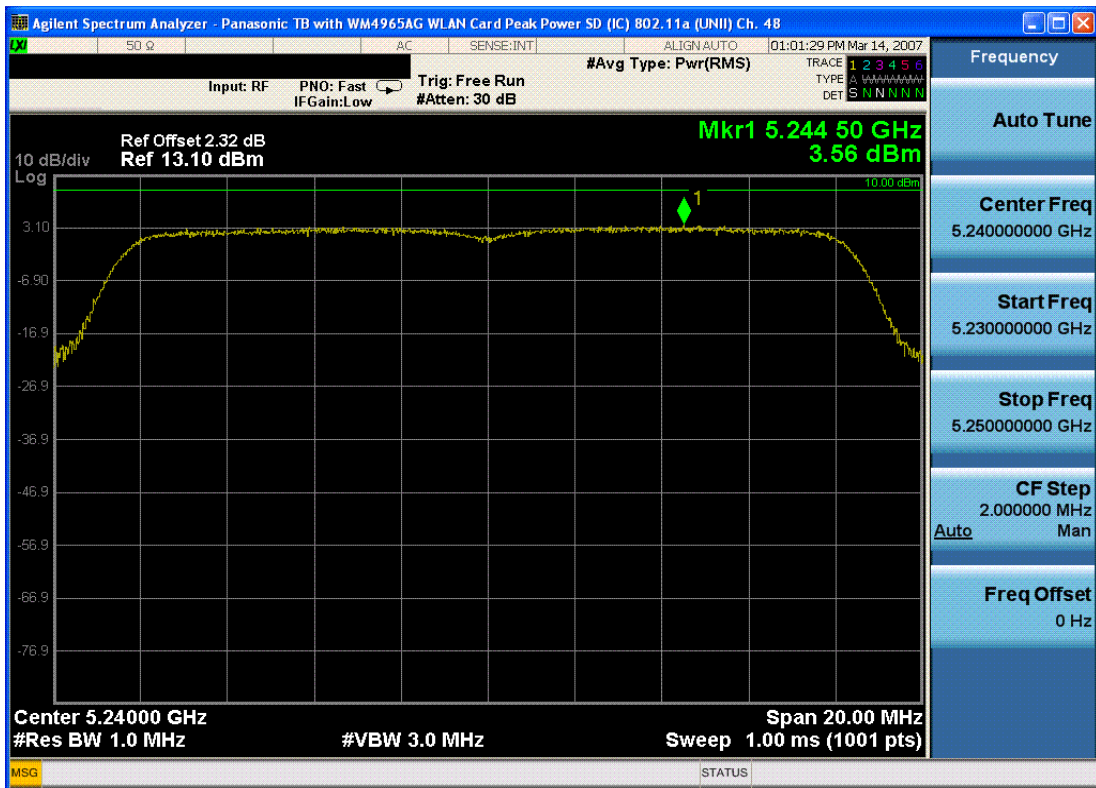
Plot 6-9. Peak Power Spectral Density Plot [Industry Canada] (802.11a (UNII) – Ch. 48)
