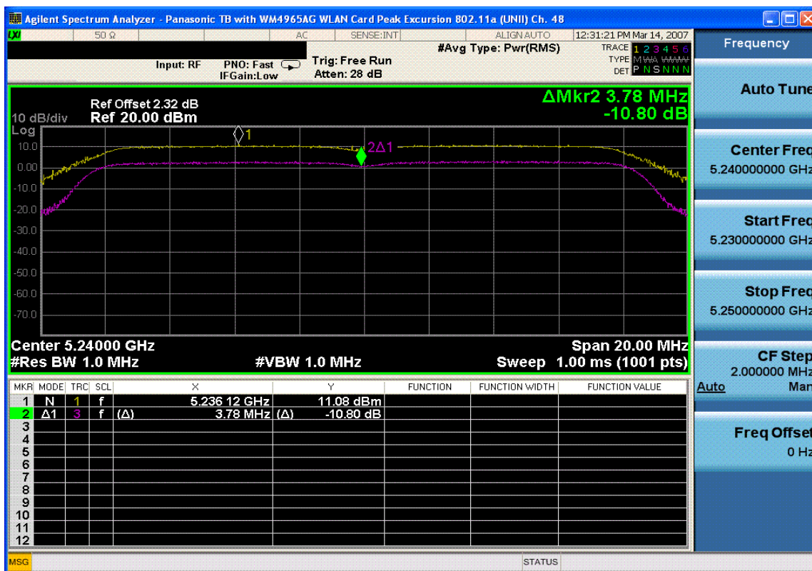
Plot 6-12. Peak Excursion Ratio Plot (802.11a (UNII) – Ch. 48)
