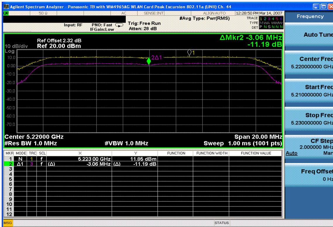
Plot 6-11. Peak Excursion Ratio Plot (802.11a (UNII) – Ch. 44)
