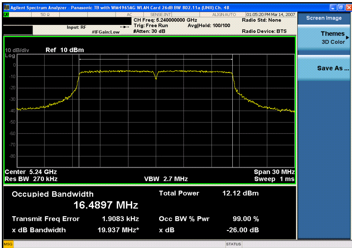
Plot 6-3. 26dB Bandwidth Plot (802.11a (UNII) – Ch. 48)
