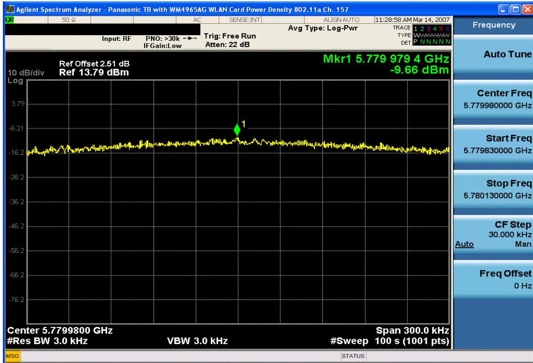
Plot 6-11. Power Spectral Density Plot (802.11a – Ch. 157)
