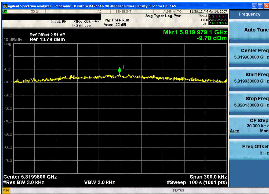
Plot 6-12. Power Spectral Density Plot (802.11a – Ch. 165)
