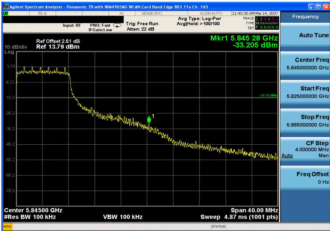
Plot 6-16. Band Edge Plot (802.11a – Ch. 165)
