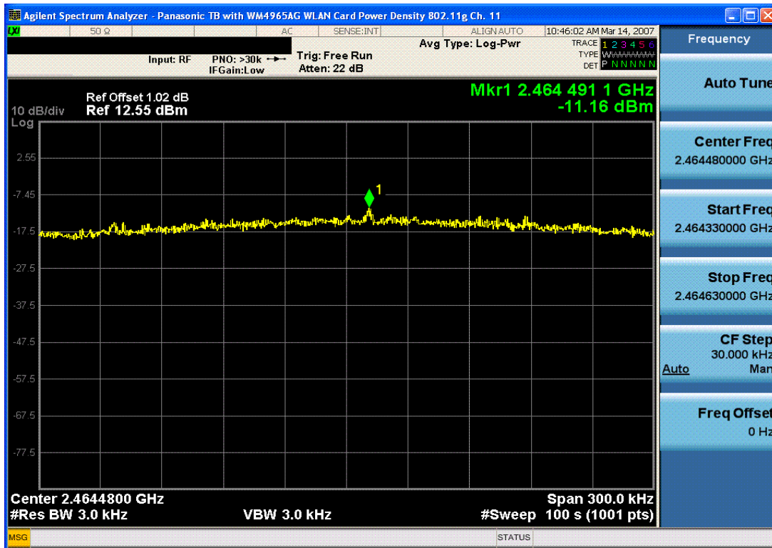
Plot 6-9. Power Spectral Density Plot (802.11g – Ch. 11)
