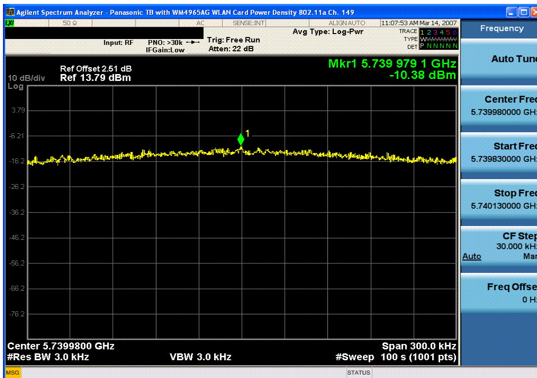
Plot 6-10. Power Spectral Density Plot (802.11a – Ch. 149)
