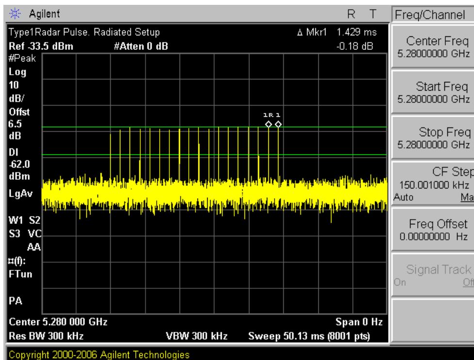
Figure 5-8. Radar Type1 Pulse
