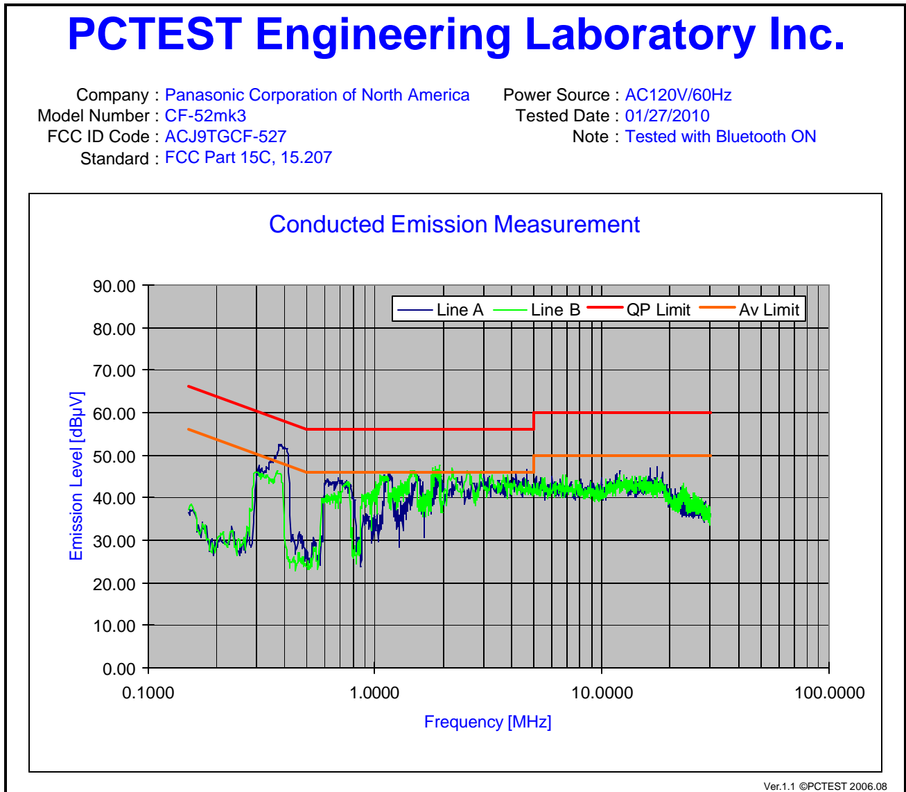
Plot 6-18. Line Conducted Plot with Bluetooth
