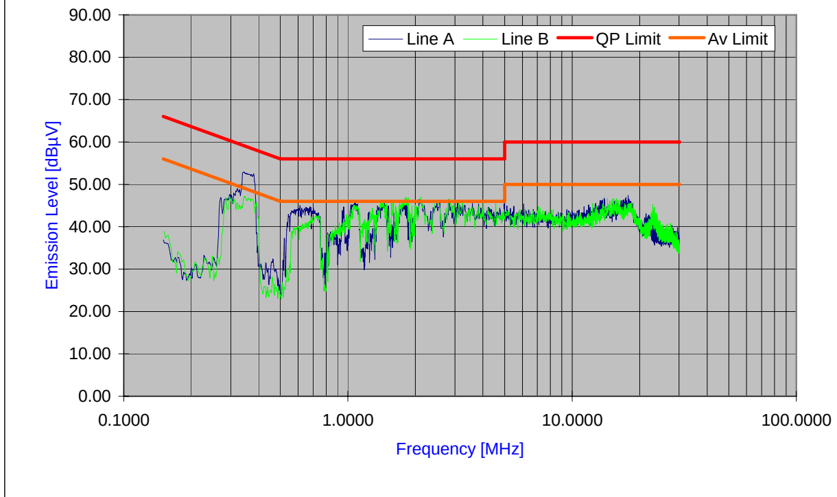
Plot 6-92. Line Conducted Plot with 802.11a (UNII Band III)
