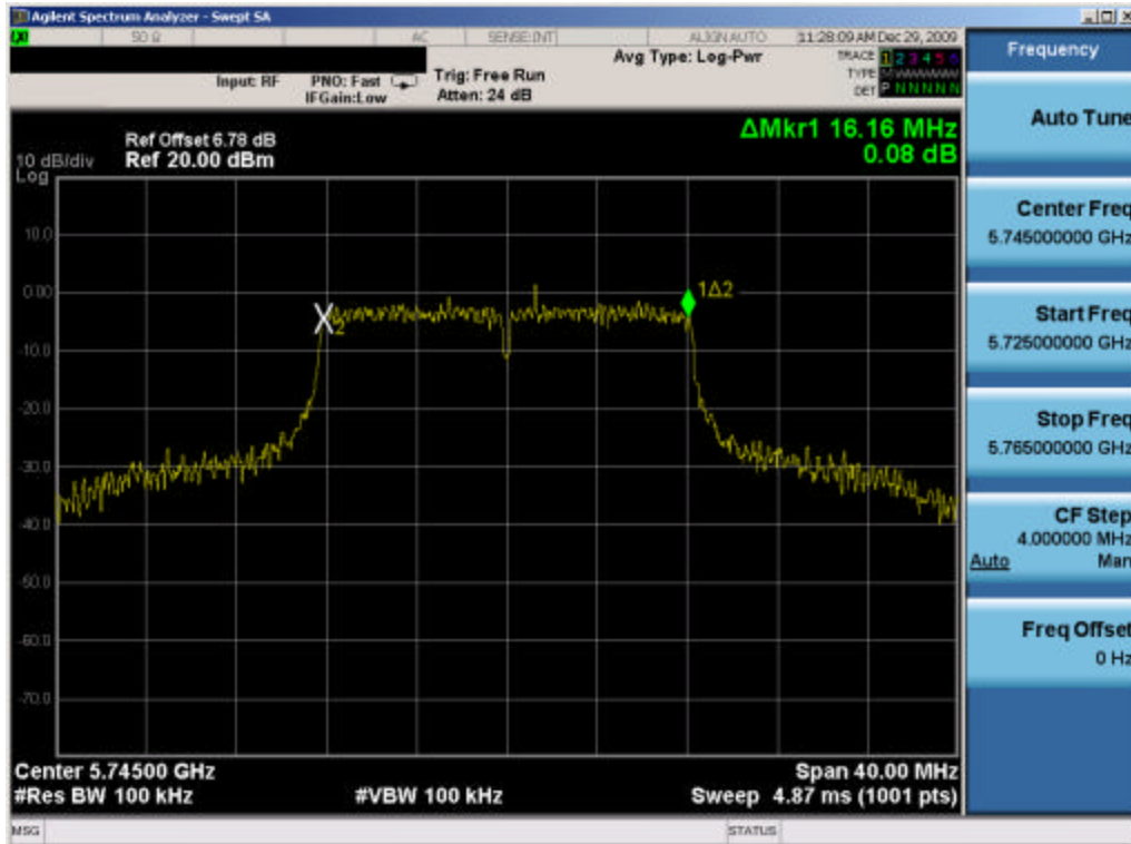
Plot 6-7. 6dB Bandwidth Plot (802.11a – Ch. 149) – Chain A
