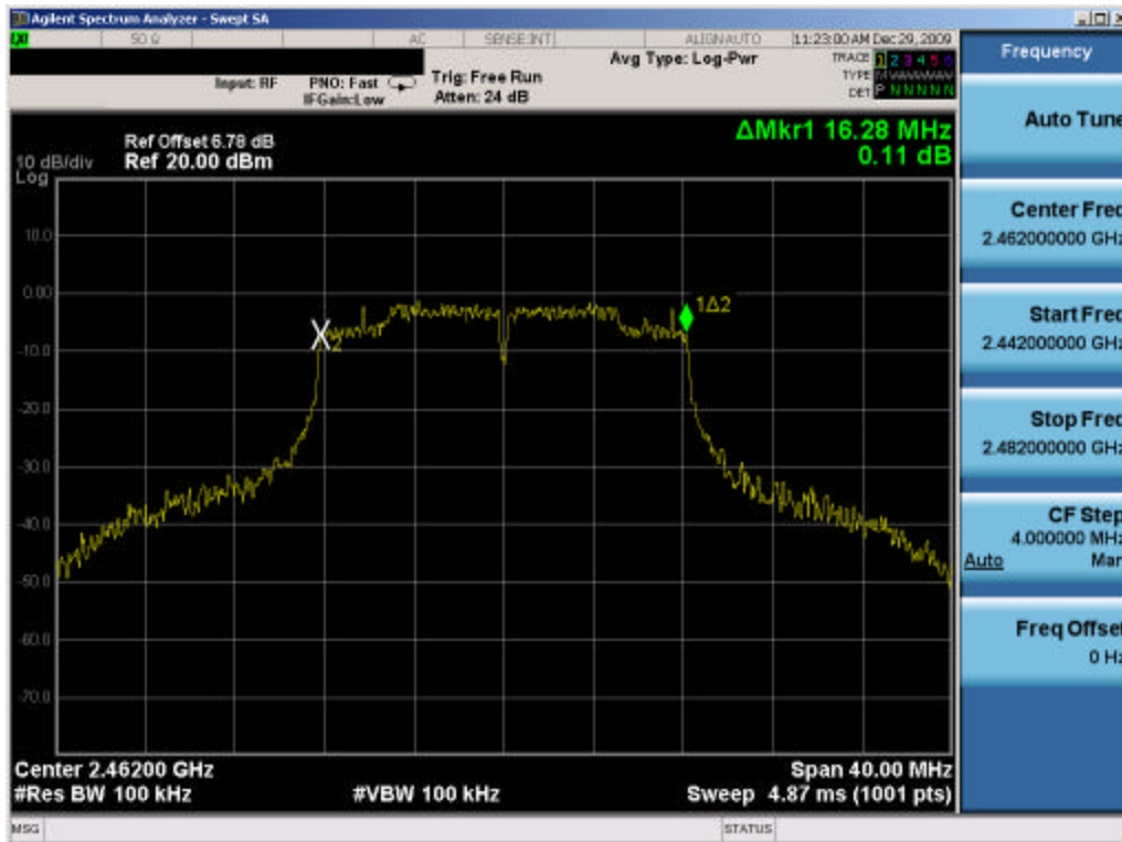
Plot 6-6. 6dB Bandwidth Plot (802.11g – Ch. 11) – Chain A
