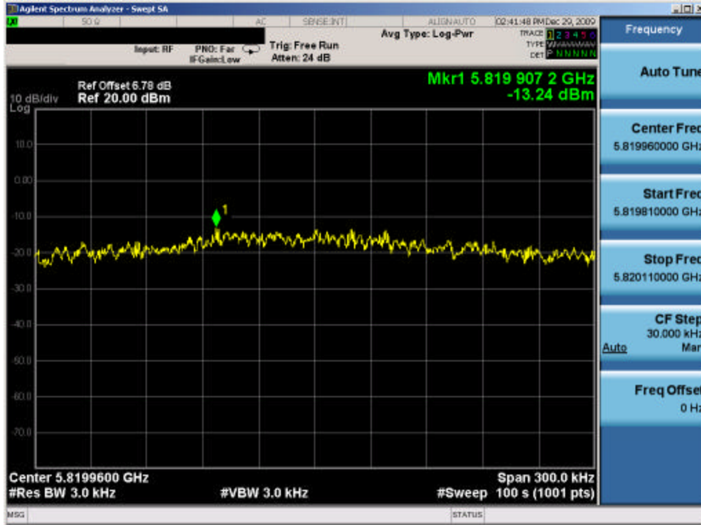
Plot 6-37. Power Spectral Density Plot (802.11a – Ch. 165) – Chain A
