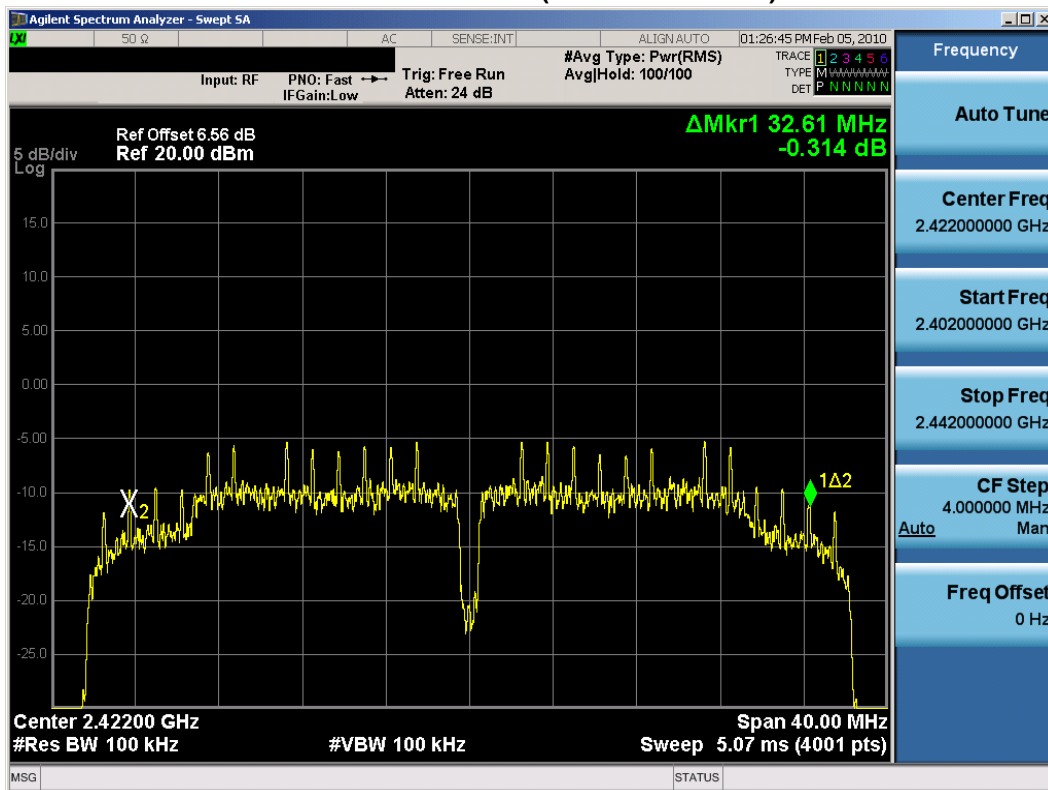
Plot 6-24. 6dB Bandwidth Plot (802.11n (2.4GHz) – Ch. 3) – Chain B
