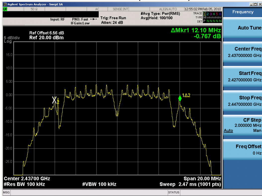
Plot 6-16. 6dB Bandwidth Plot (802.11b – Ch. 6) – Chain B
