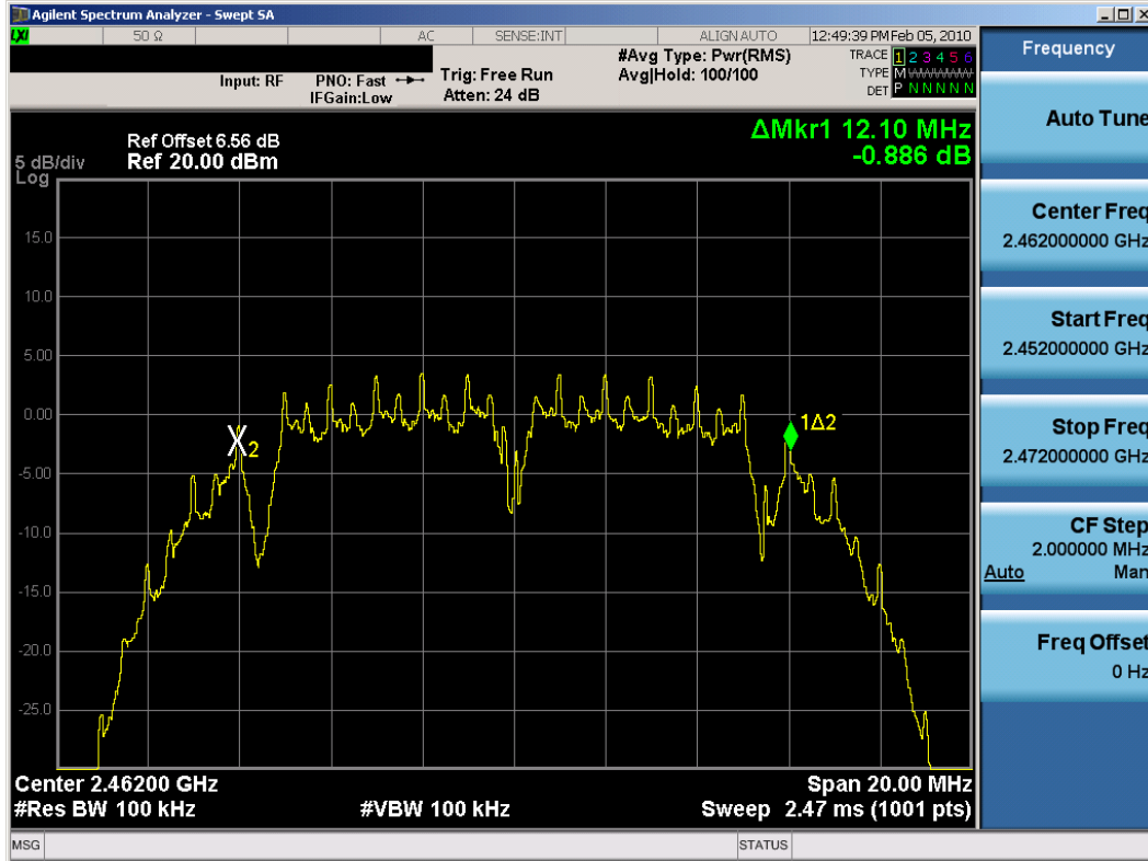
Plot 6-17. 6dB Bandwidth Plot (802.11b – Ch. 11) – Chain B
