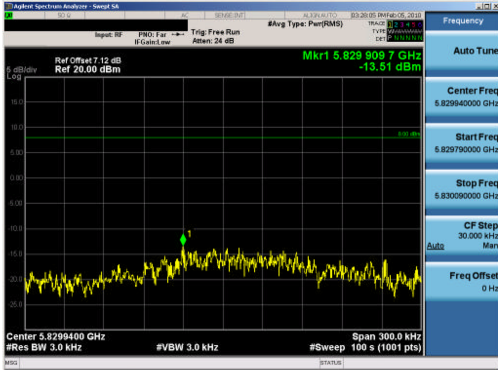
Plot 6-51. Power Spectral Density Plot (802.11a – Ch. 165) – Chain B
