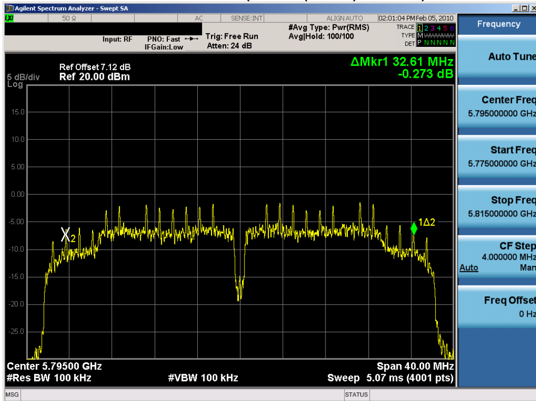
Plot 6-28. 6dB Bandwidth Plot (802.11n (5.8GHz) – Ch. 159) – Chain B
