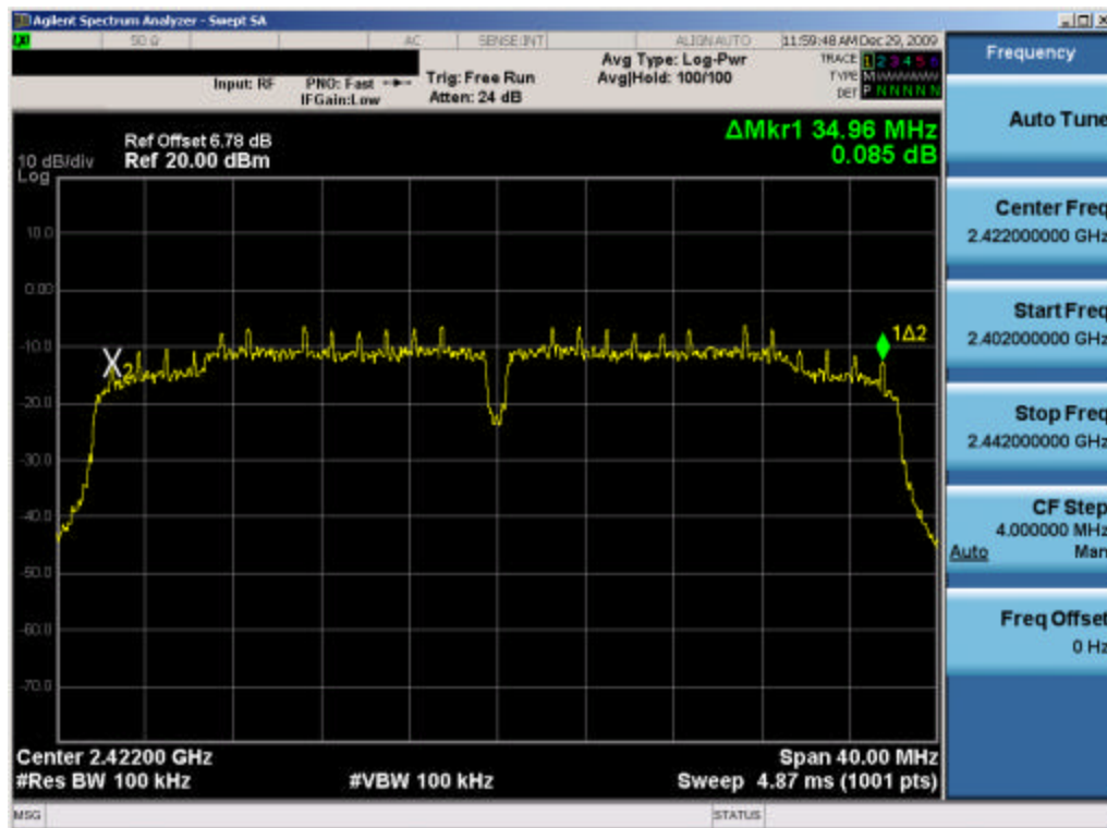
Plot 6-10. 6dB Bandwidth Plot (802.11n (2.4GHz) – Ch. 3) – Chain A
