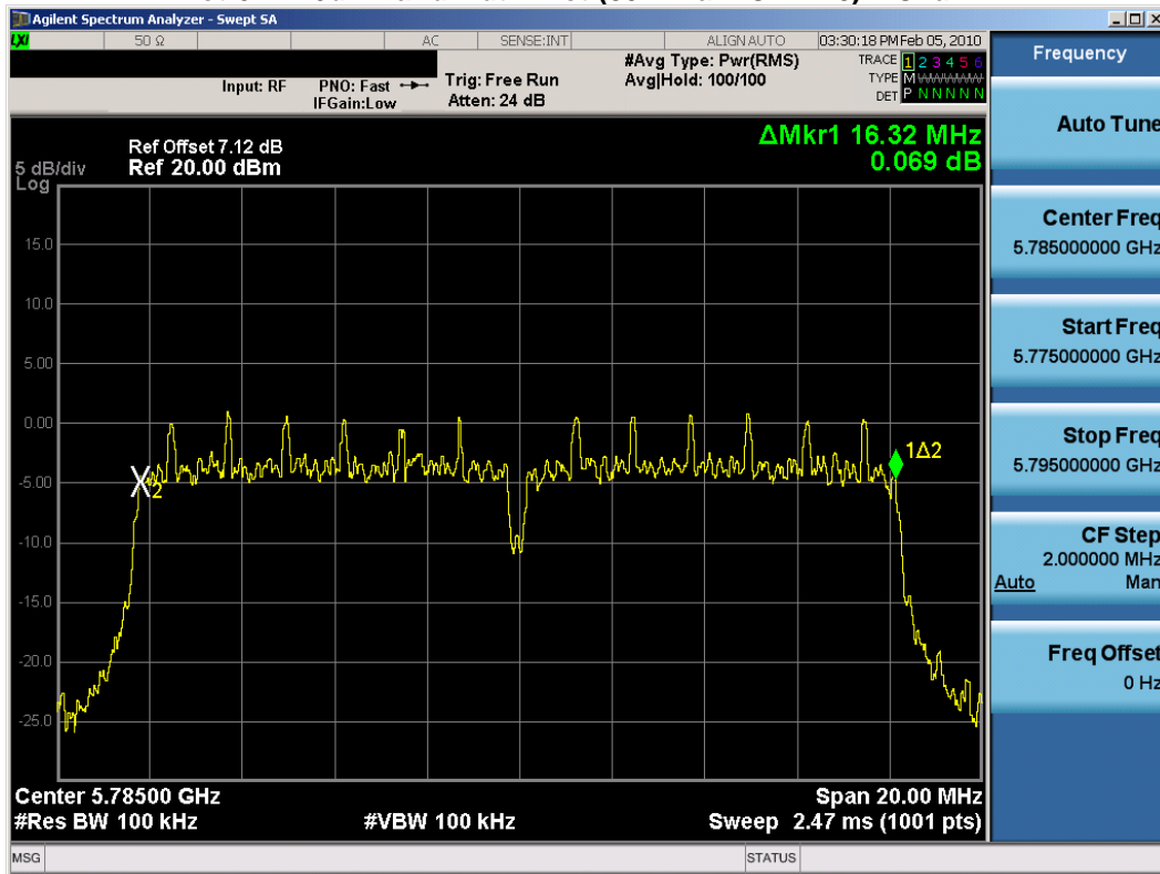
Plot 6-22. 6dB Bandwidth Plot (802.11a – Ch. 157) – Chain B
