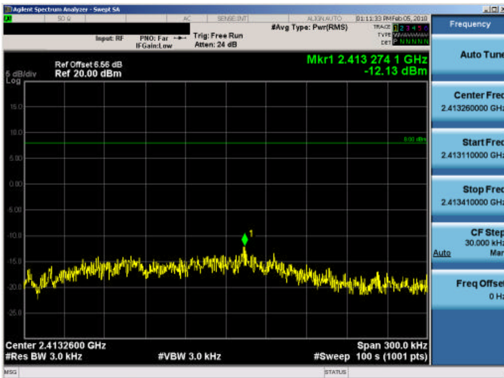
Plot 6-46. Power Spectral Density Plot (802.11g – Ch. 1) – Chain B
