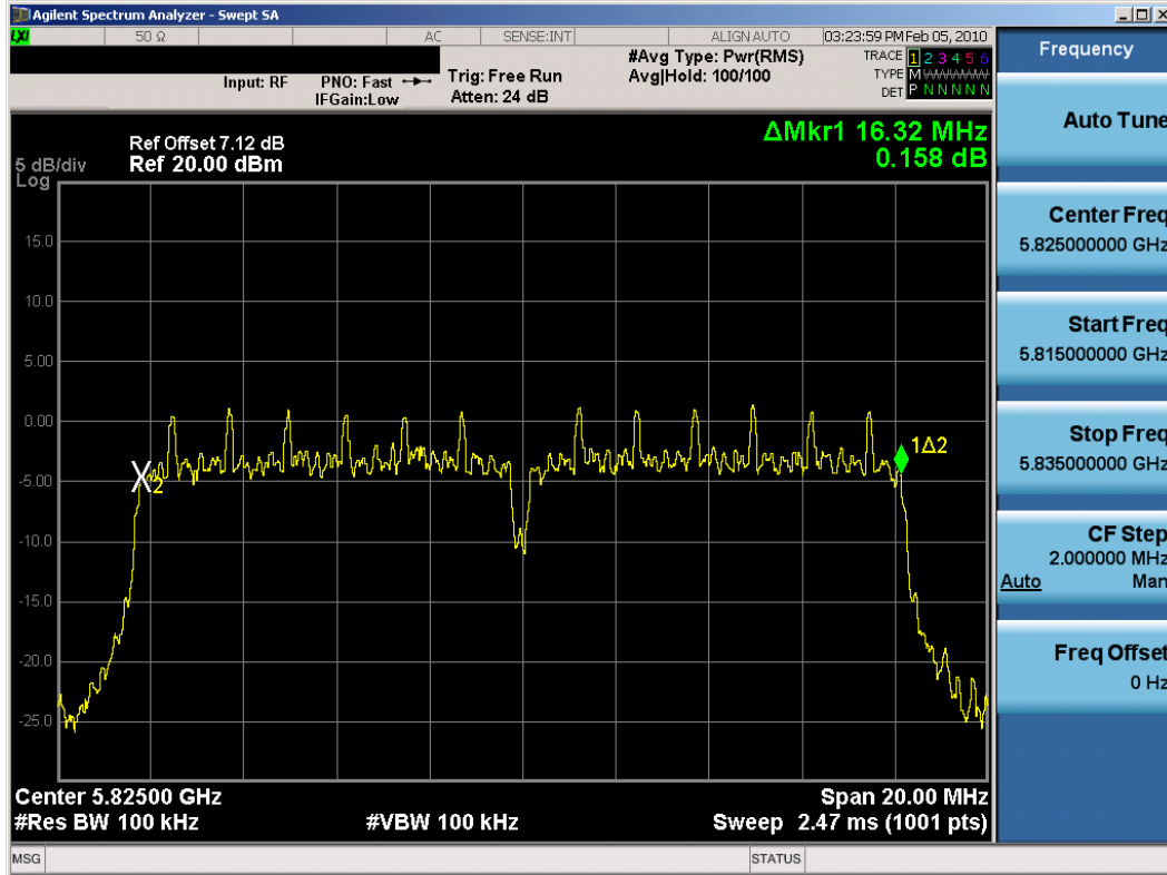
Plot 6-23. 6dB Bandwidth Plot (802.11a – Ch. 165) – Chain B
