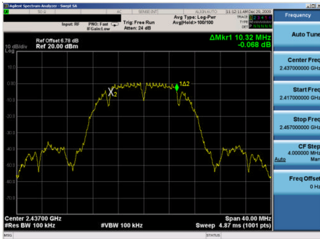
Plot 6-2. 6dB Bandwidth Plot (802.11b – Ch. 6) – Chain A
