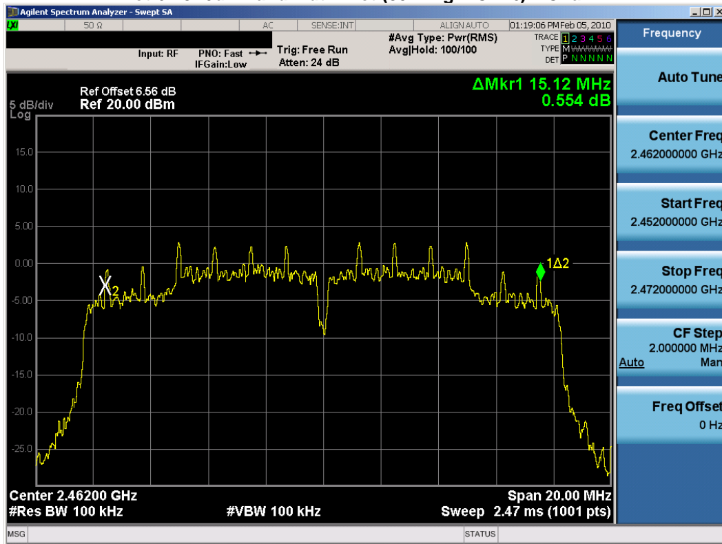
Plot 6-20. 6dB Bandwidth Plot (802.11g – Ch. 11) – Chain B
