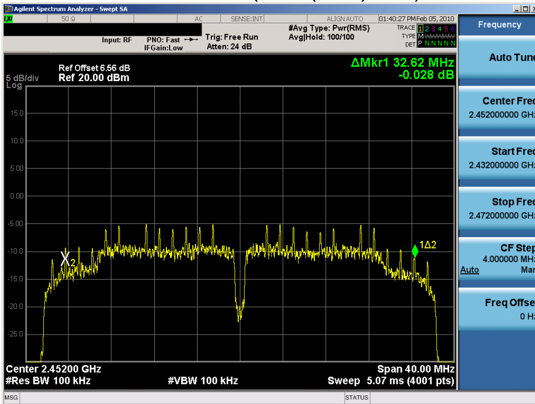
Plot 6-26. 6dB Bandwidth Plot (802.11n (2.4GHz) – Ch. 9) – Chain B
