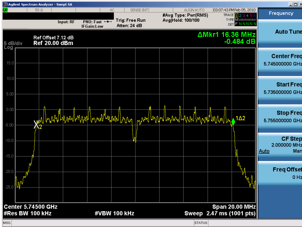
Plot 6-21. 6dB Bandwidth Plot (802.11a – Ch. 149) – Chain B
