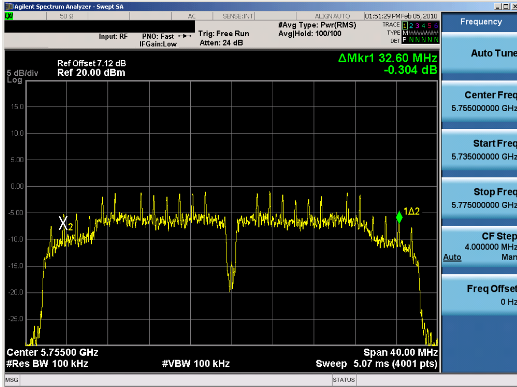
Plot 6-27. 6dB Bandwidth Plot (802.11n (5.8GHz) – Ch. 151) – Chain B
