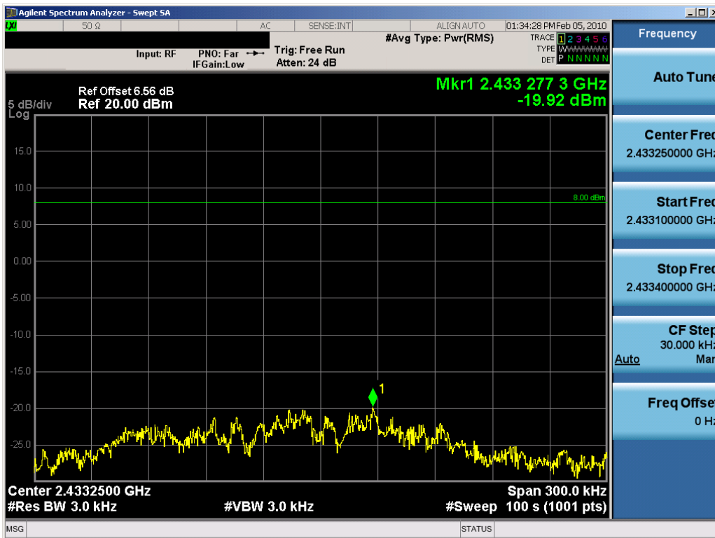
Plot 6-52. Power Spectral Density Plot (802.11n (2.4GHz) – Ch. 3) – Chain B
