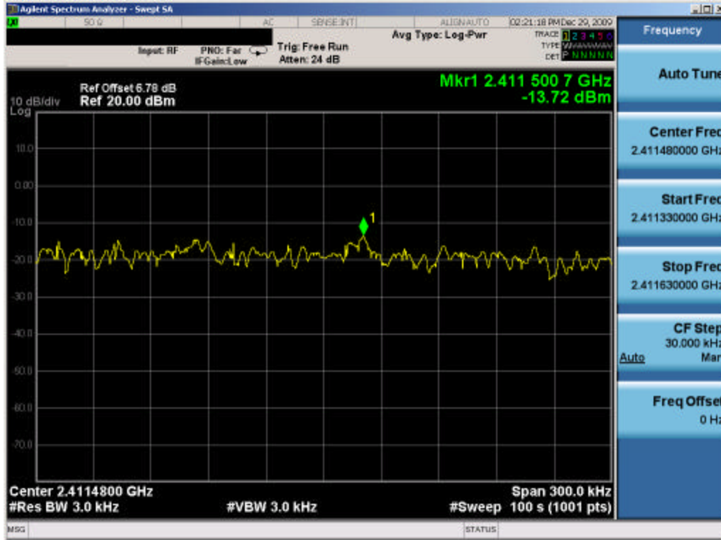
Plot 6-29. Power Spectral Density Plot (802.11b – Ch. 1) – Chain A
