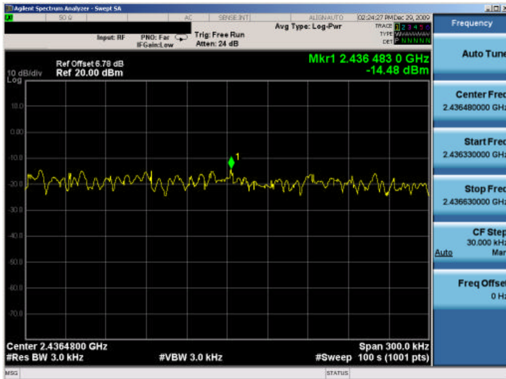
Plot 6-30. Power Spectral Density Plot (802.11b – Ch. 6) – Chain A
