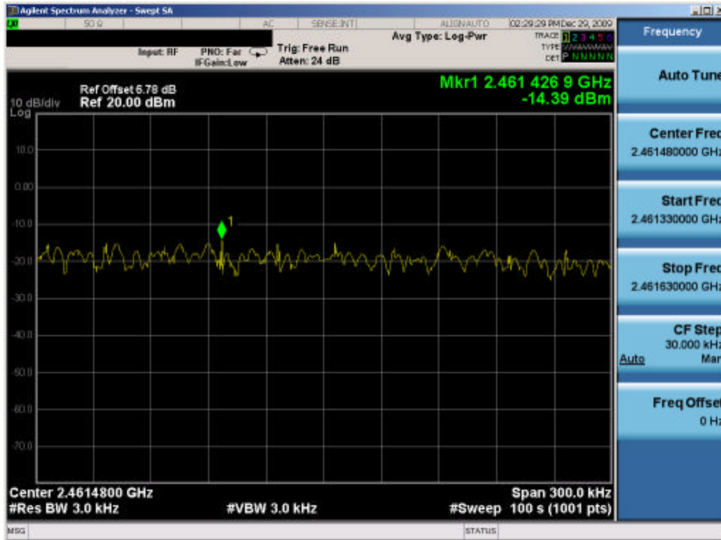
Plot 6-31. Power Spectral Density Plot (802.11b – Ch. 11) – Chain A
