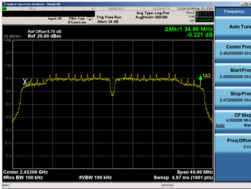
Plot 6-12. 6dB Bandwidth Plot (802.11n (2.4GHz) – Ch. 9) – Chain A
