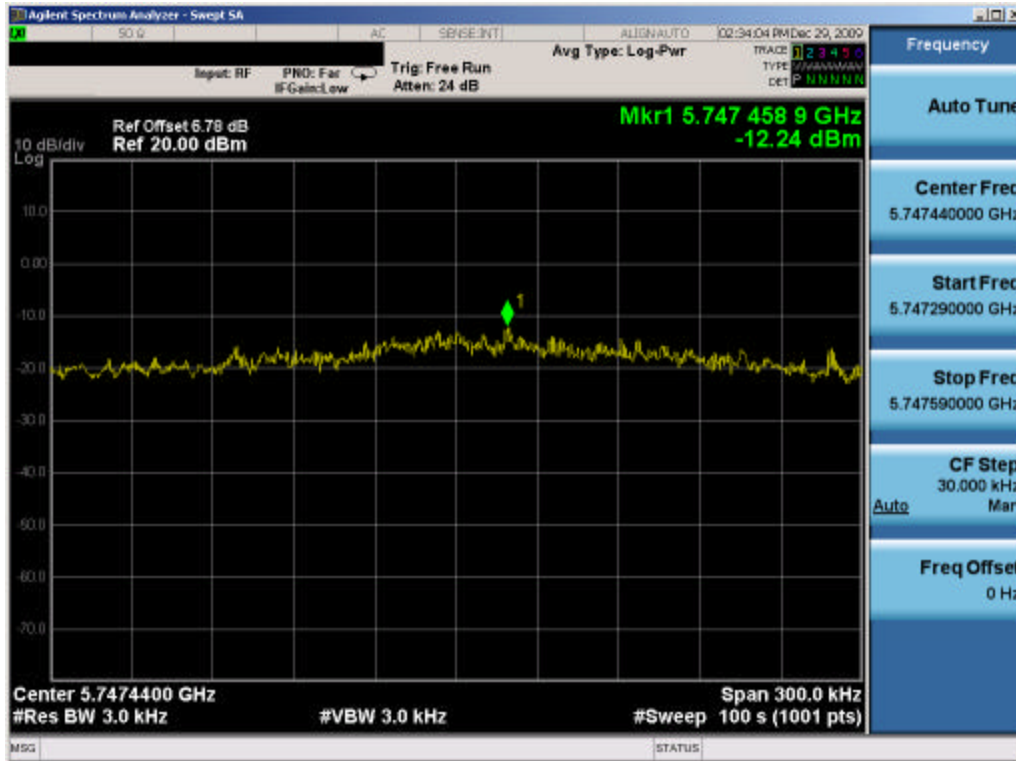
Plot 6-35. Power Spectral Density Plot (802.11a – Ch. 149) – Chain A
