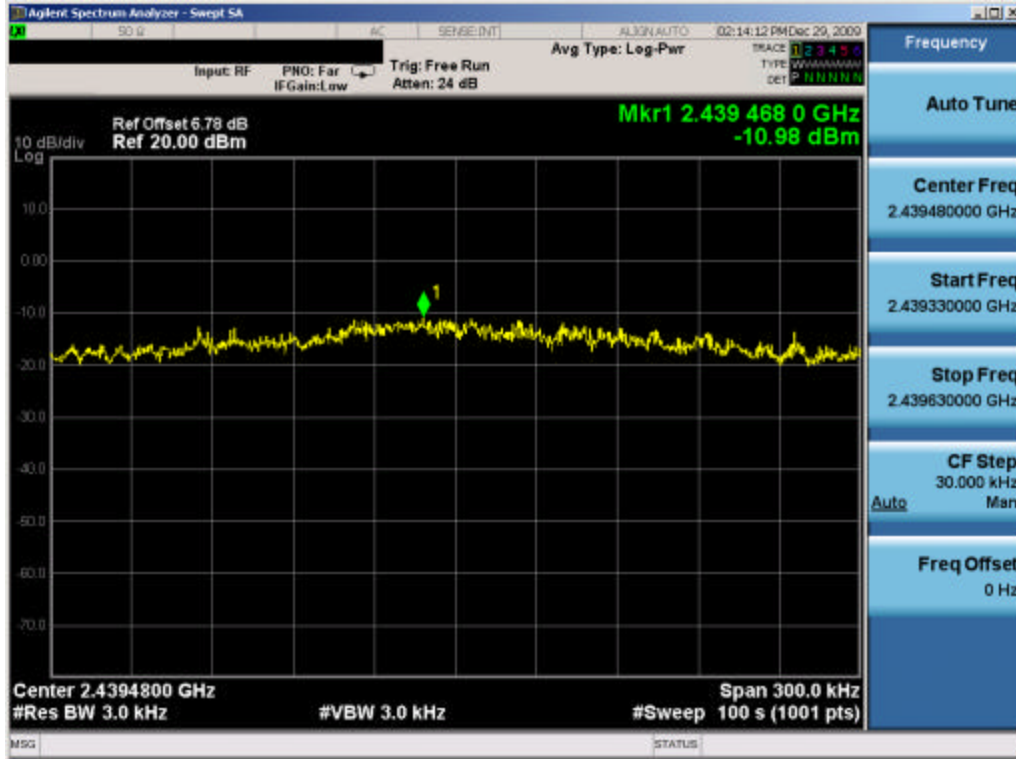
Plot 6-33. Power Spectral Density Plot (802.11g – Ch. 6) – Chain A
