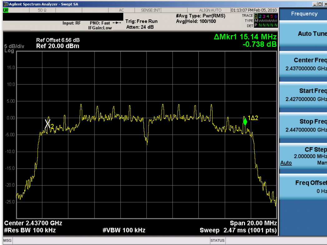
Plot 6-19. 6dB Bandwidth Plot (802.11g – Ch. 6) – Chain B
