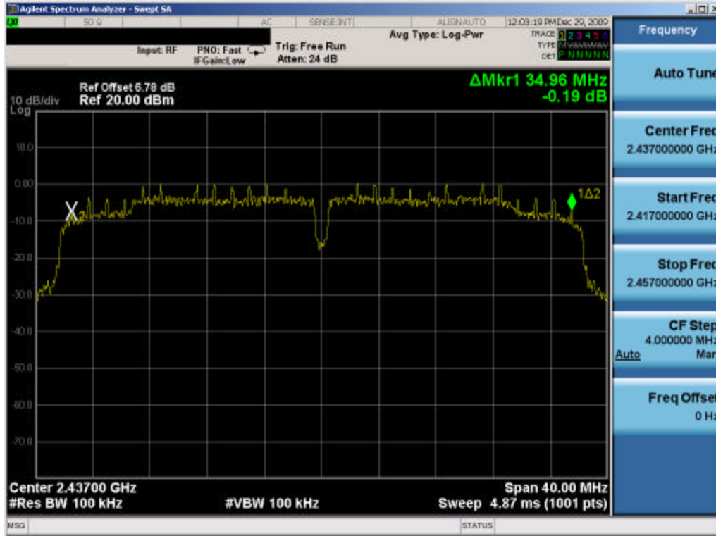
Plot 6-11. 6dB Bandwidth Plot (802.11n (2.4GHz) – Ch. 6) – Chain A
