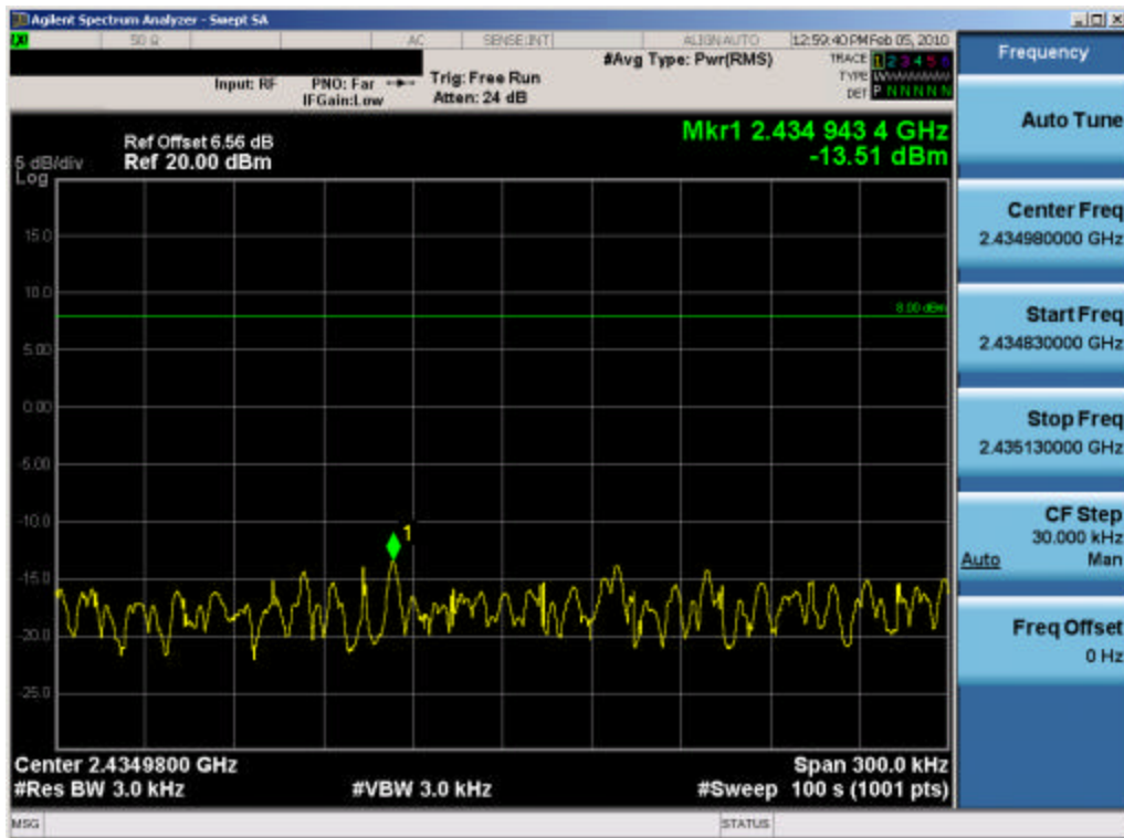
Plot 6-44. Power Spectral Density Plot (802.11b – Ch. 6) – Chain B
