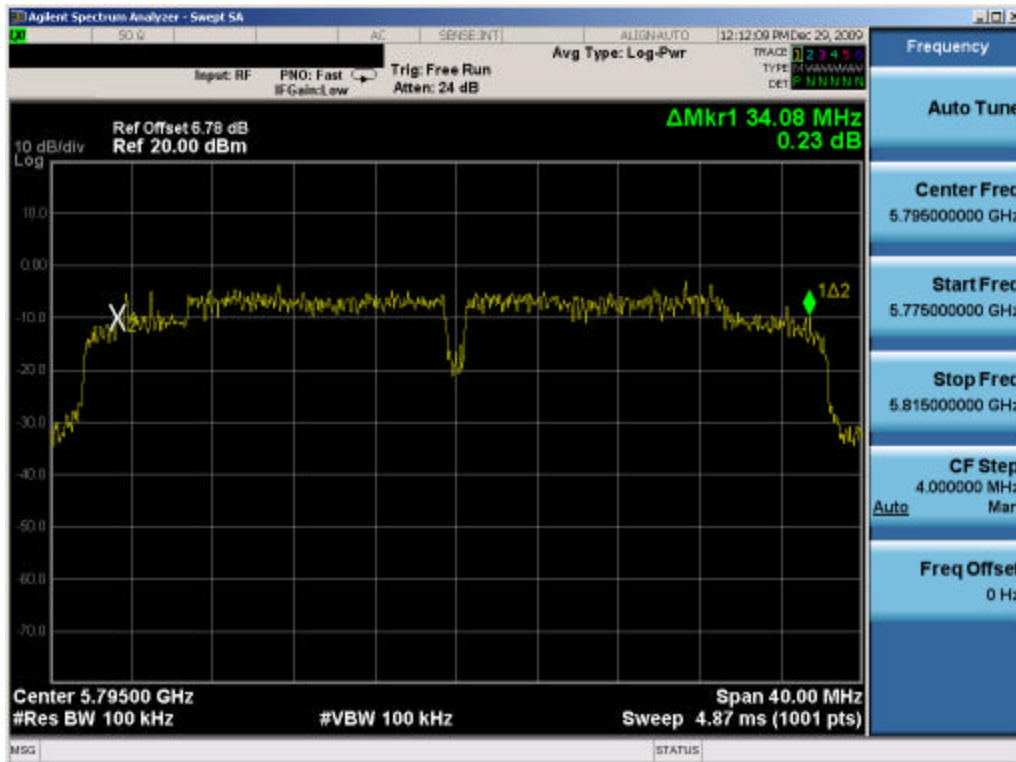
Plot 6-14. 6dB Bandwidth Plot (802.11n (5.8GHz) – Ch. 159) – Chain A
