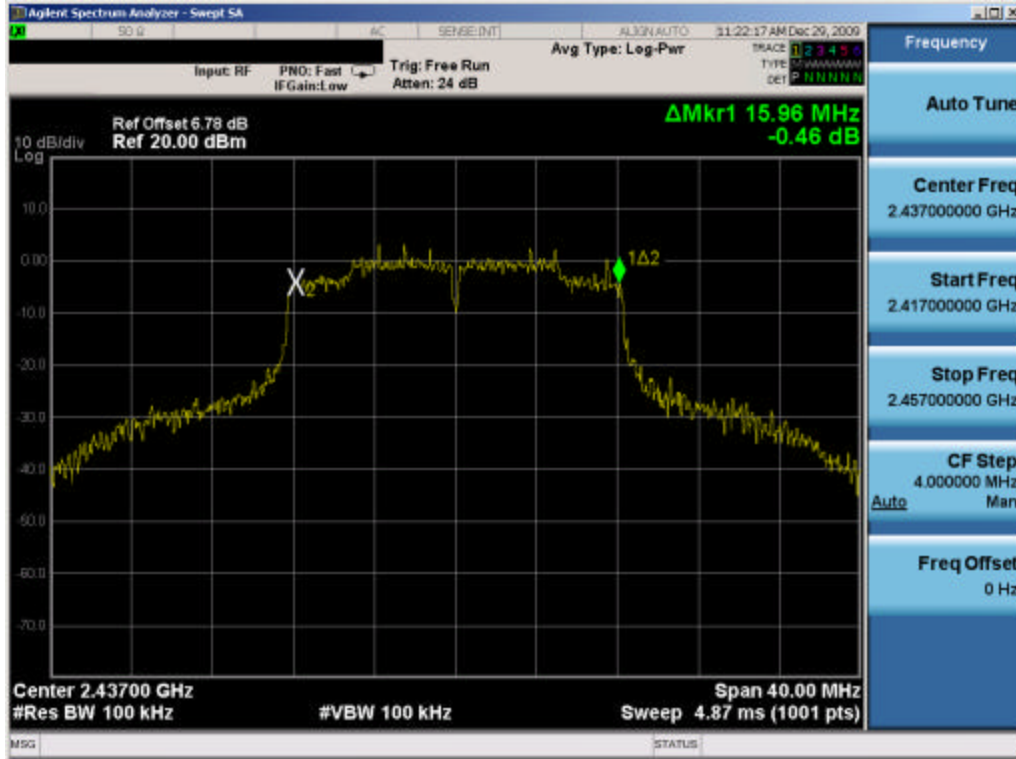
Plot 6-5. 6dB Bandwidth Plot (802.11g – Ch. 6) – Chain A
