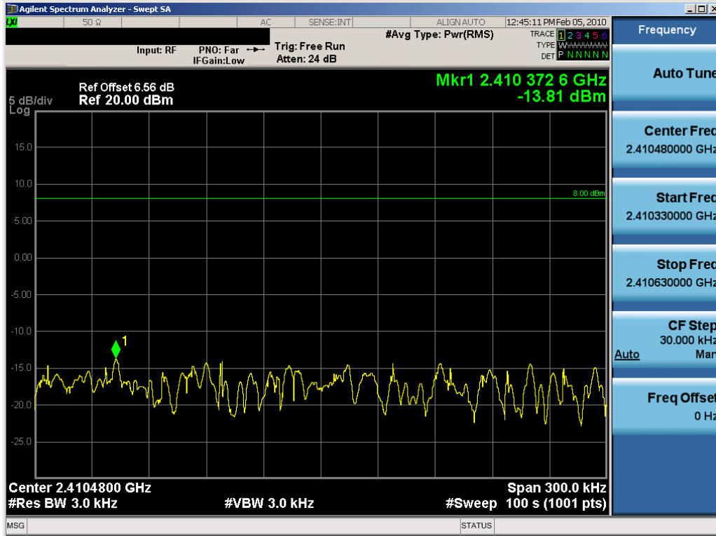
Plot 6-43. Power Spectral Density Plot (802.11b – Ch. 1) – Chain B
