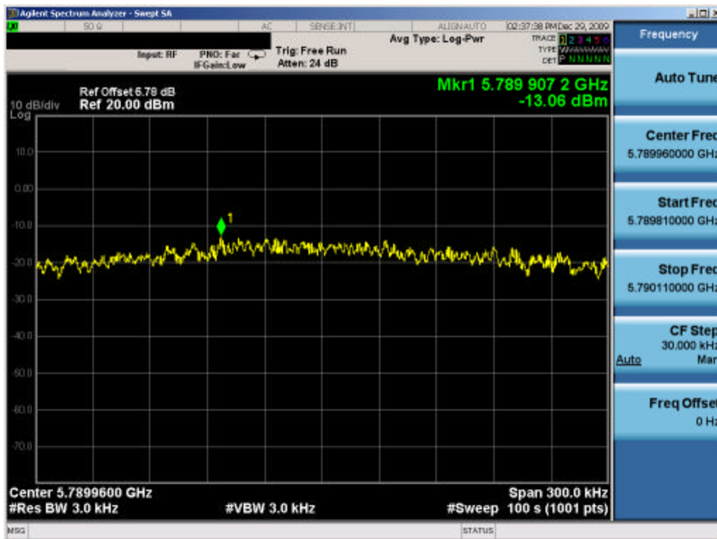
Plot 6-36. Power Spectral Density Plot (802.11a – Ch. 157) – Chain A
