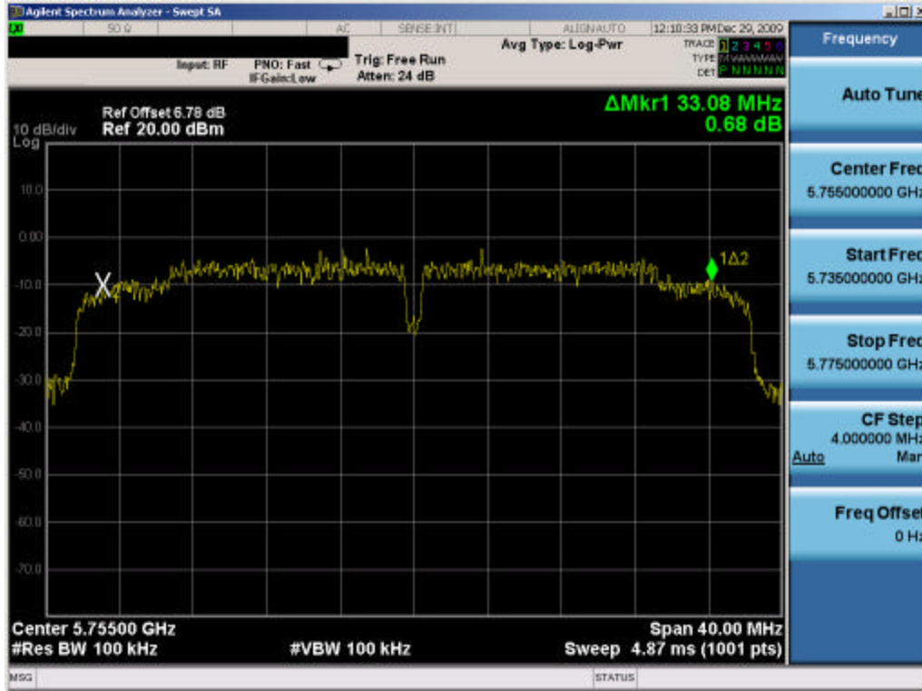
Plot 6-13. 6dB Bandwidth Plot (802.11n (5.8GHz) – Ch. 151) – Chain A
