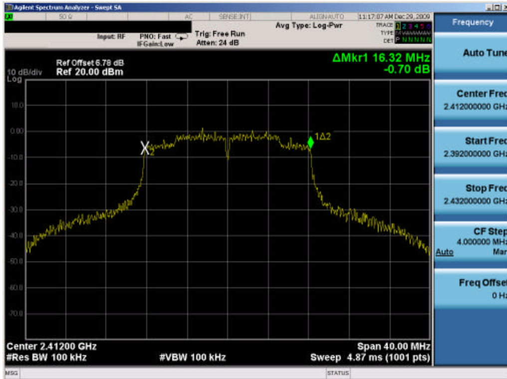
Plot 6-4. 6dB Bandwidth Plot (802.11g – Ch. 1) – Chain A
