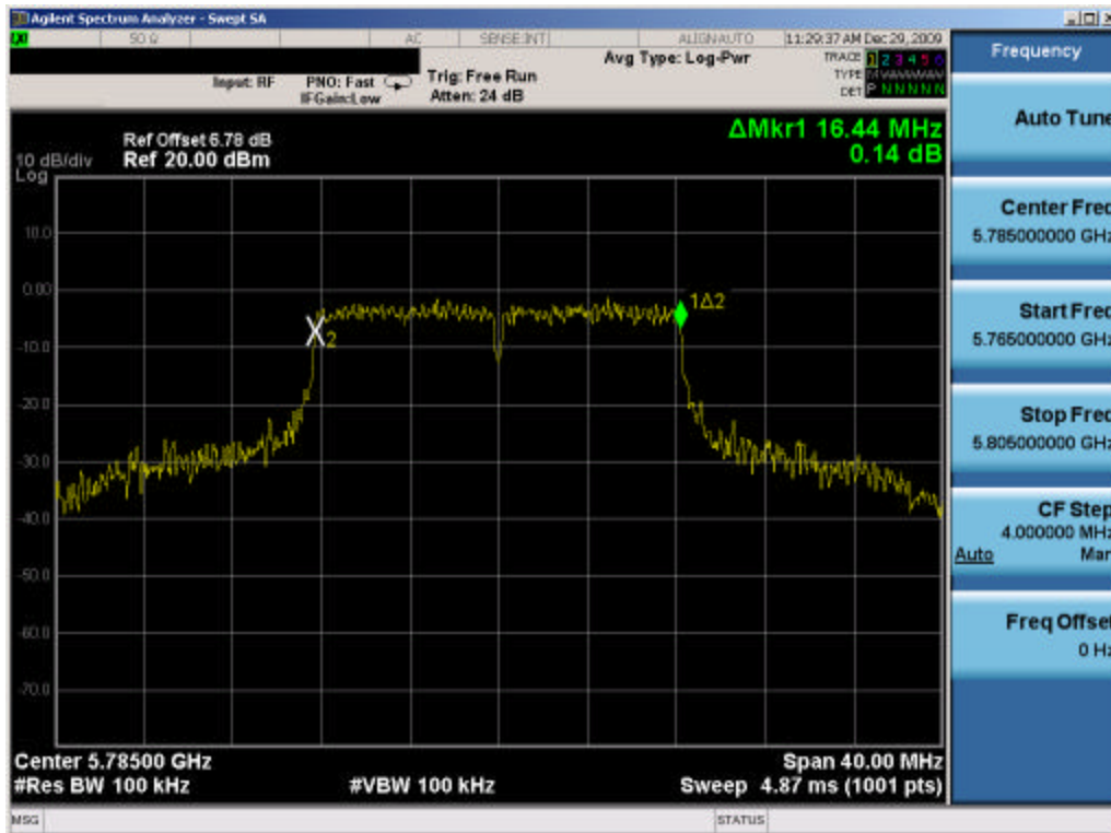
Plot 6-8. 6dB Bandwidth Plot (802.11a – Ch. 157) – Chain A
