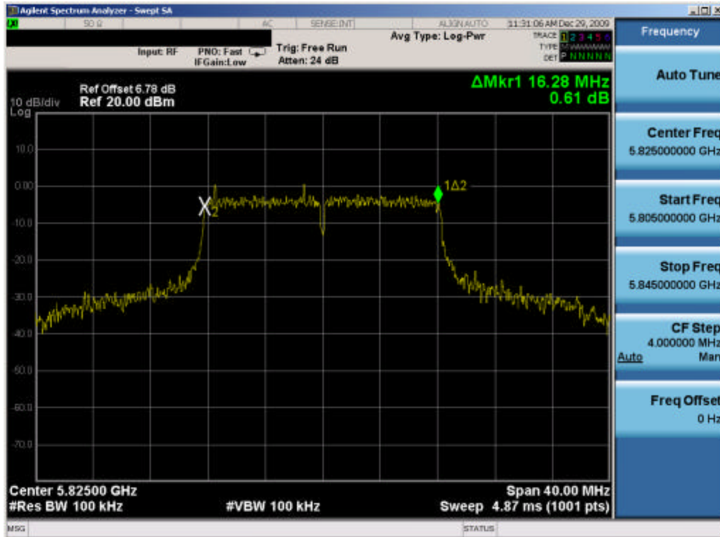
Plot 6-9. 6dB Bandwidth Plot (802.11a – Ch. 165) – Chain A
