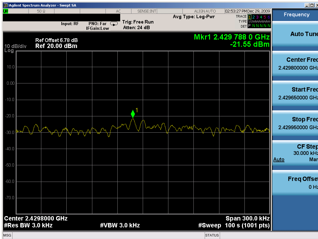
Plot 6-38. Power Spectral Density Plot (802.11n (2.4GHz) – Ch. 3) – Chain A
