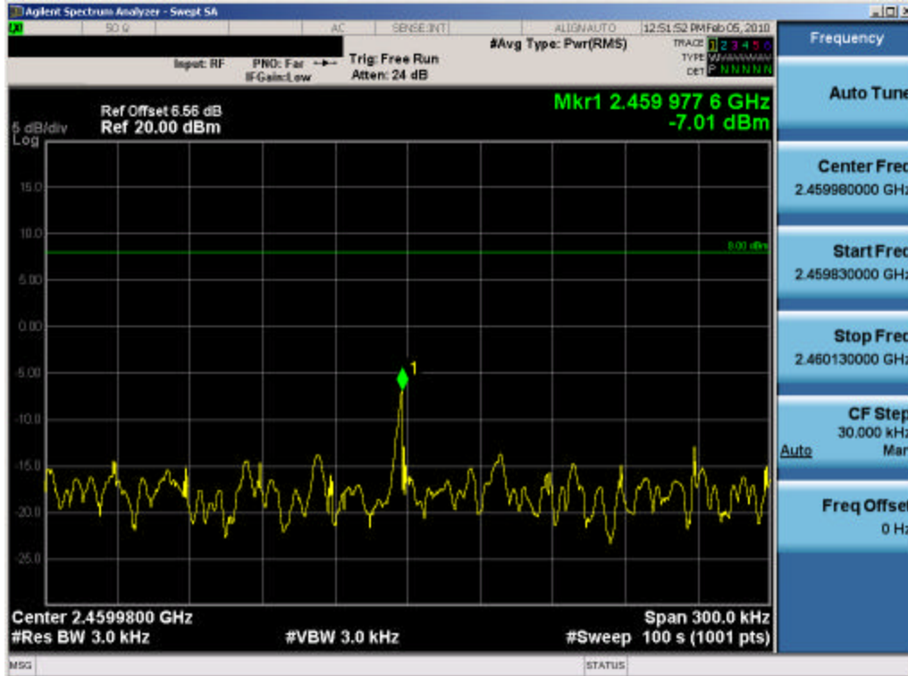
Plot 6-45. Power Spectral Density Plot (802.11b – Ch. 11) – Chain B
