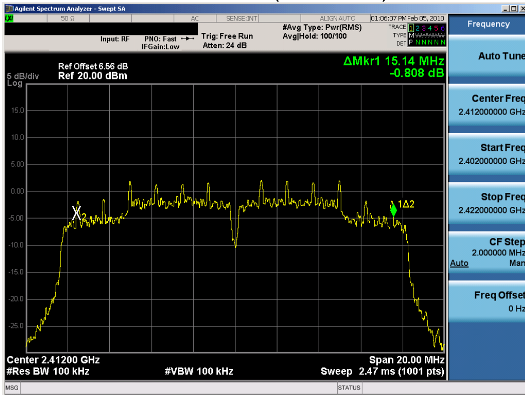
Plot 6-18. 6dB Bandwidth Plot (802.11g – Ch. 1) – Chain B
