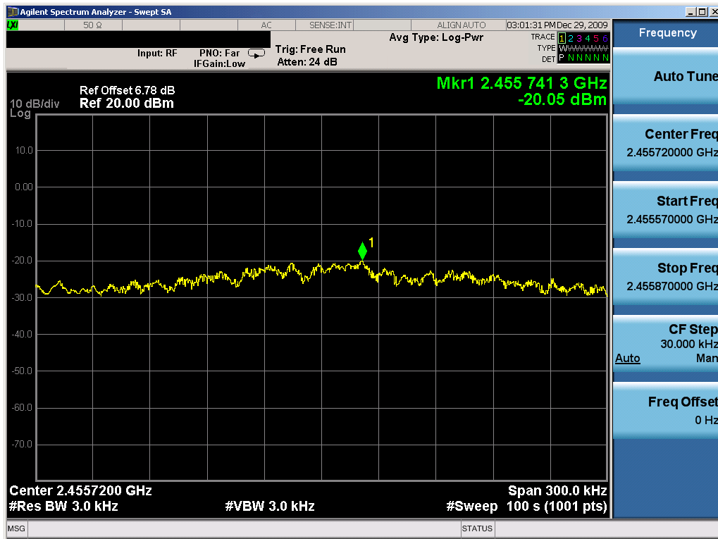
Plot 6-40. Power Spectral Density Plot (802.11n (2.4GHz) – Ch. 9) – Chain A
