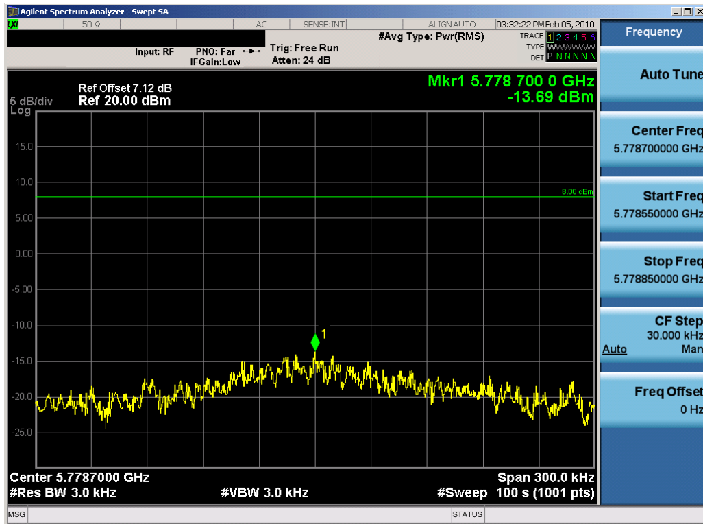
Plot 6-50. Power Spectral Density Plot (802.11a – Ch. 157) – Chain B
