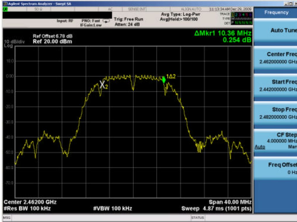
Plot 6-3. 6dB Bandwidth Plot (802.11b – Ch. 11) – Chain A
