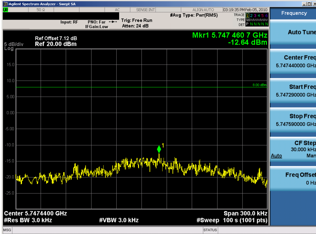
Plot 6-49. Power Spectral Density Plot (802.11a – Ch. 149) – Chain B
