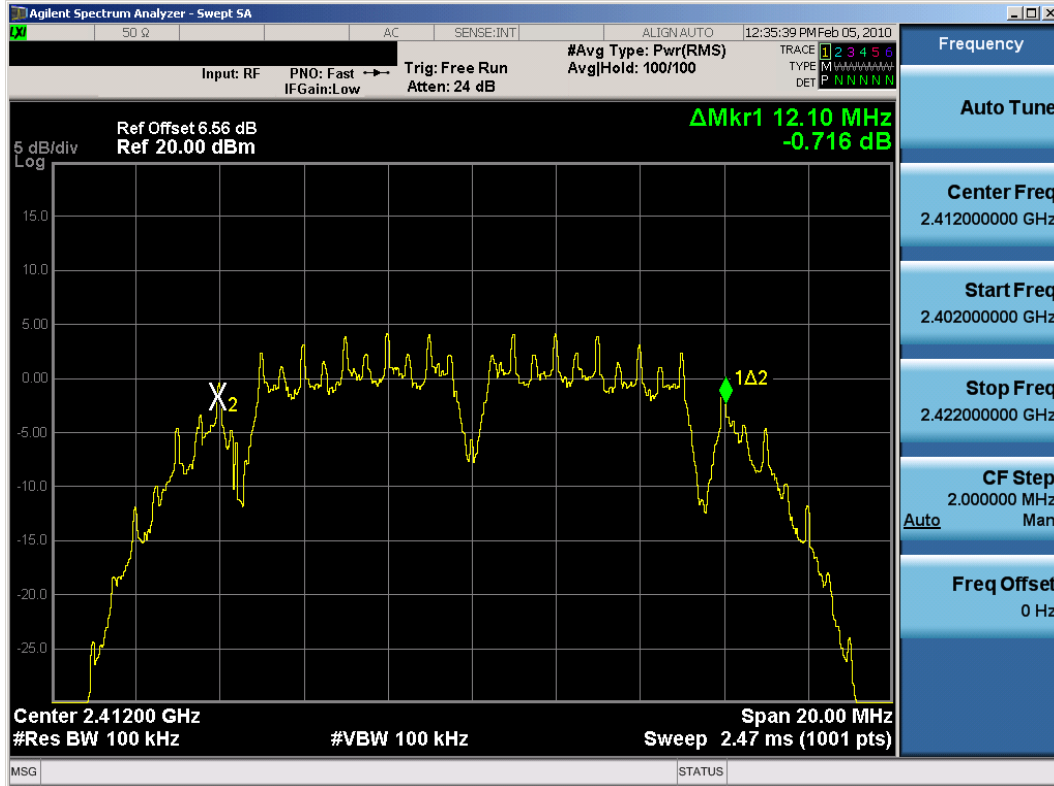
Plot 6-15. 6dB Bandwidth Plot (802.11b – Ch. 1) – Chain B
