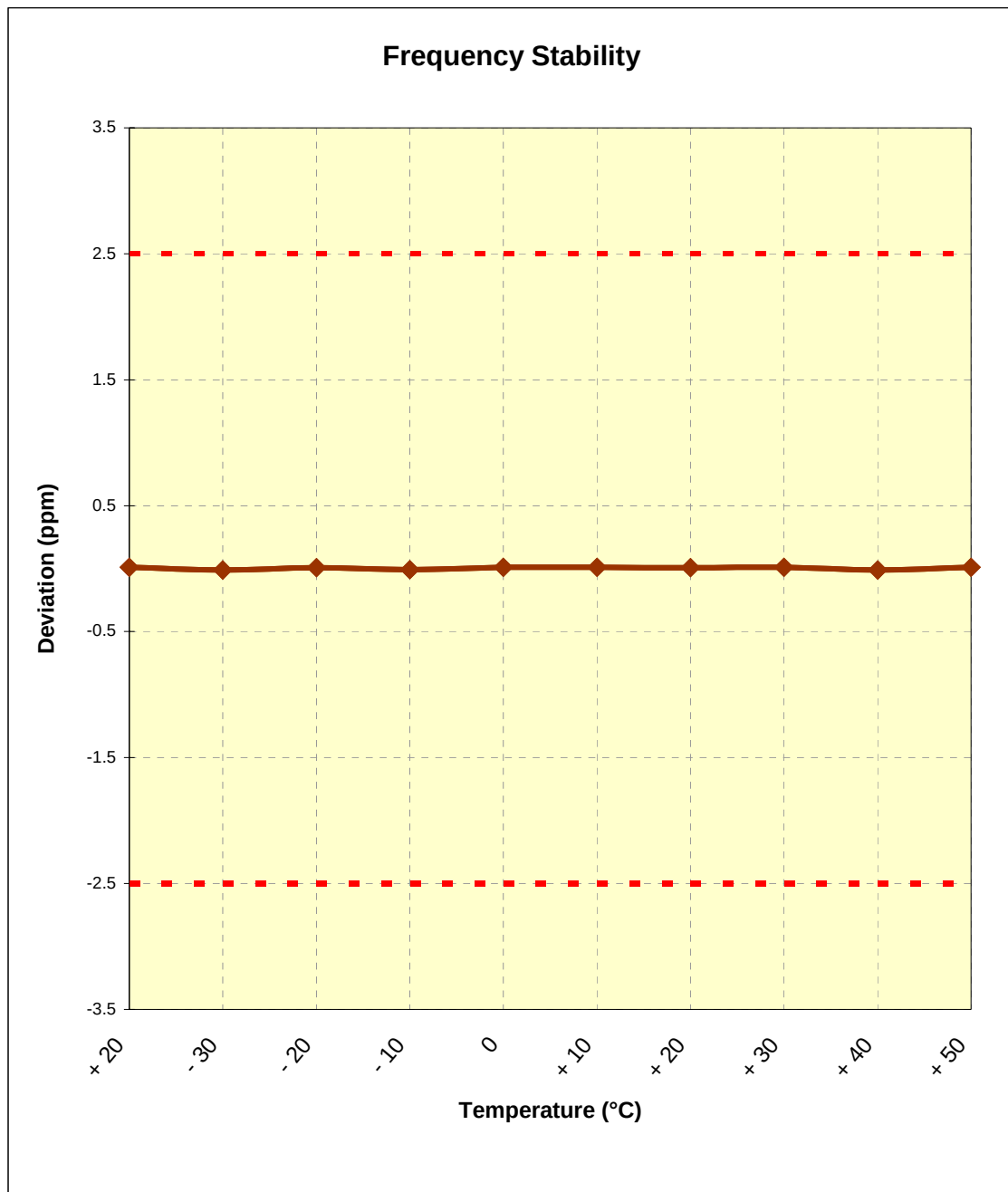
Plot 6-5. Frequency Stability Graph (PCS WCDMA Mode – Ch. 9400)
