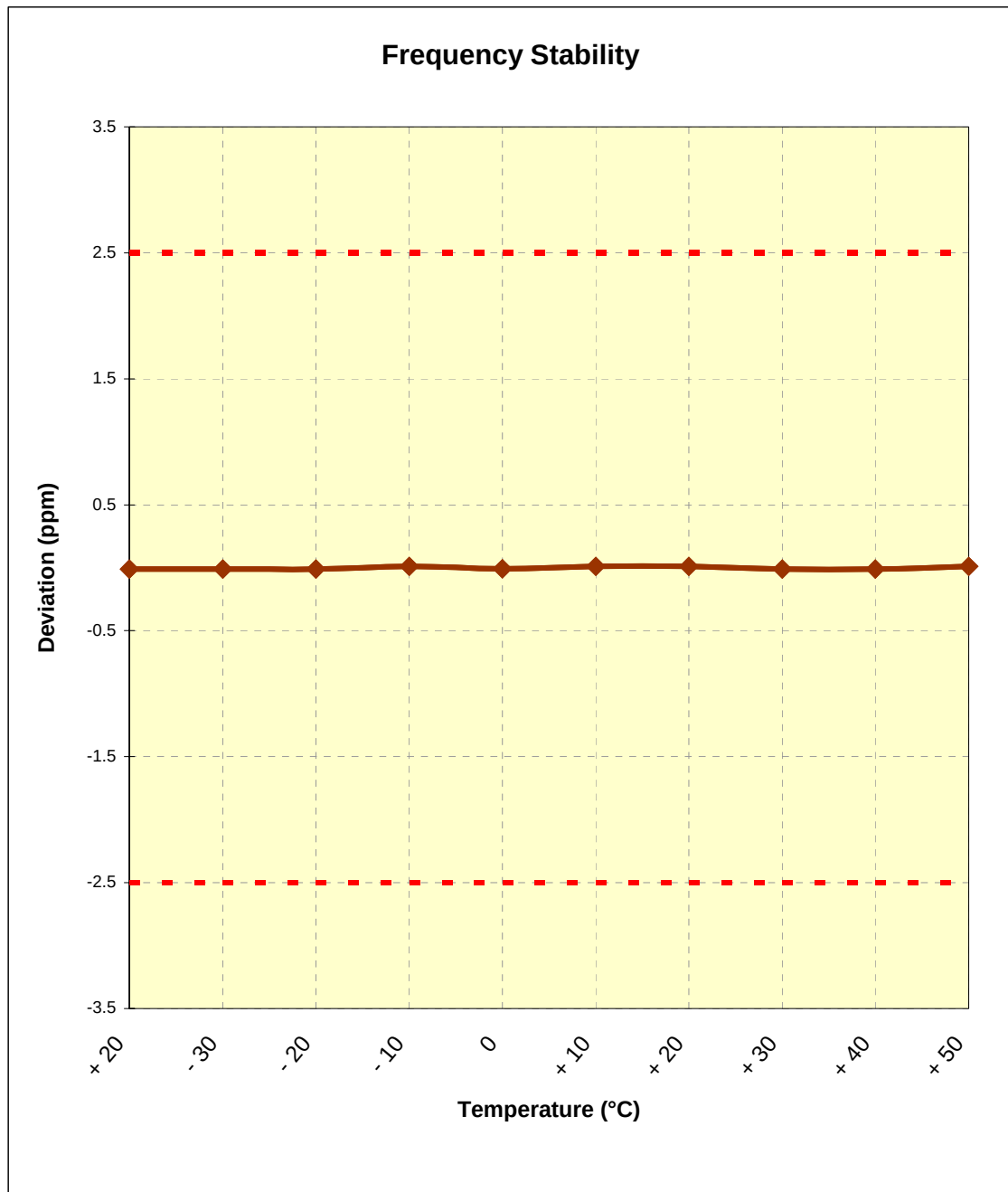
Plot 6-4. Frequency Stability Graph (PCS GSM Mode – Ch. 661)
