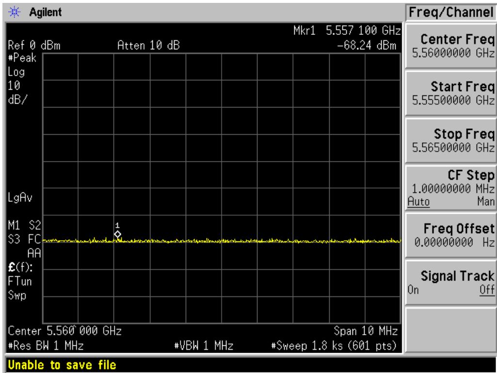
Non-occupancy Period – 30 Minute Plot (5500 – 5700MHz Band)
