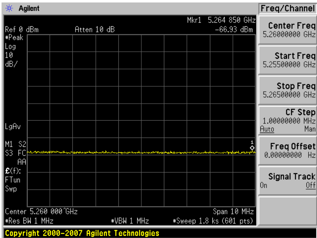
Non-occupancy Period – 30 Minute Plot (5260 – 5320MHz Band)
