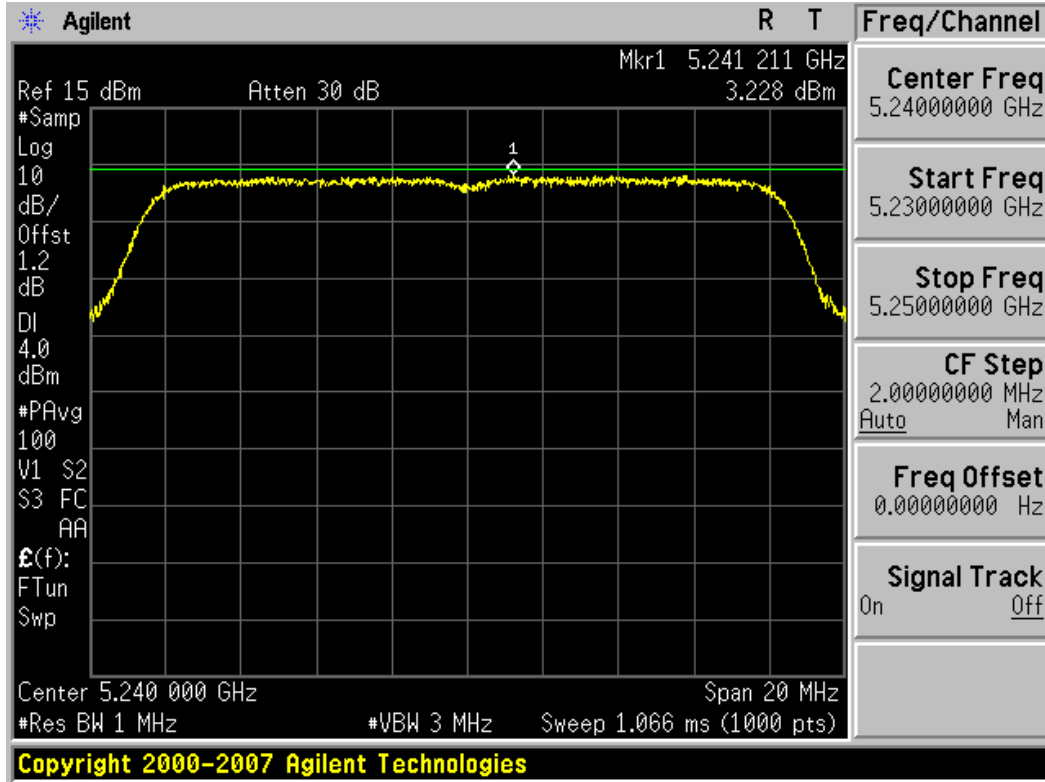
Plot 6-19. Peak Power Spectral Density Plot (802.11a (UNII) – Ch. 48)
