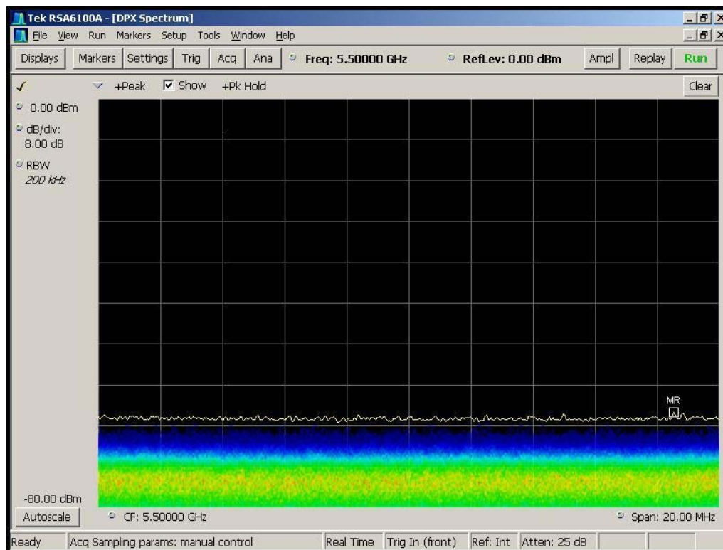
Figure 5-4 Non-occupancy Period – Monitoring live real time spectrum – elapsed time 30 minutes
