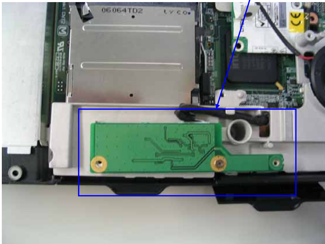
Bluetooth Card Magnified View (Main PWB removed)
