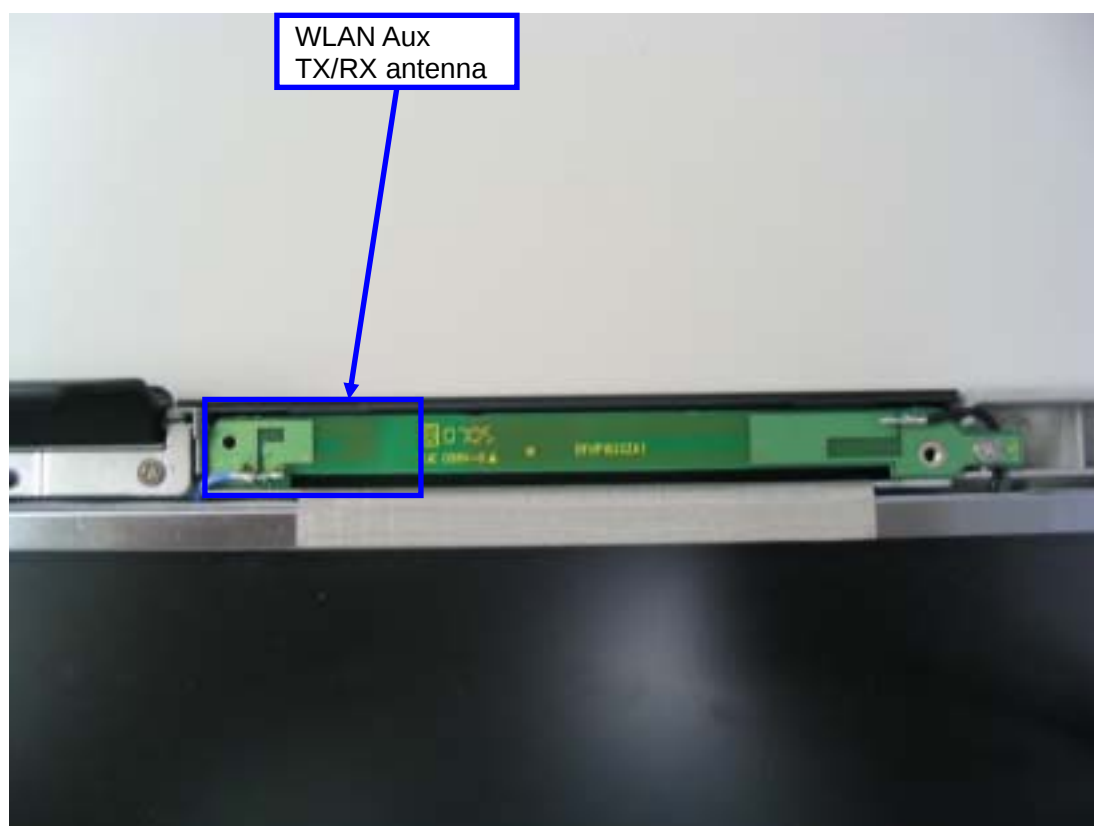
WLAN Aux antenna magnified view
