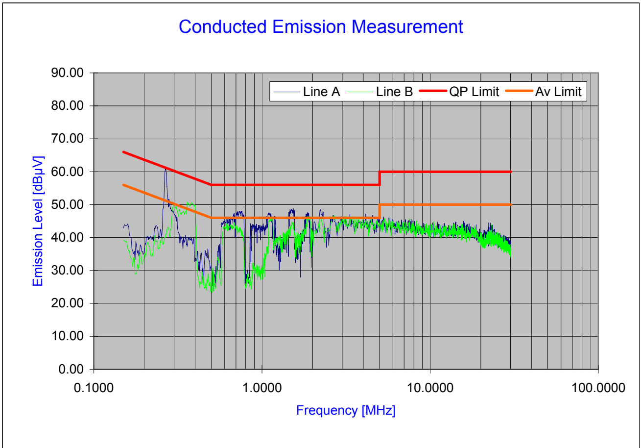
Plot 6-51. Line Conducted Plot with 802.11b
