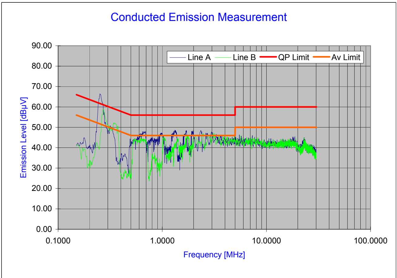
Plot 6-54. Line Conducted Plot with 802.11n
