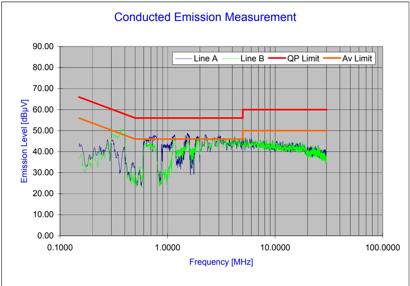
Plot 6-53. Line Conducted Plot with 802.11a
