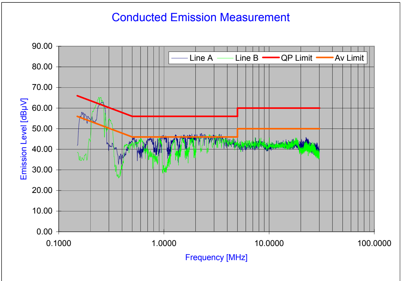
Plot 6-52. Line Conducted Plot with 802.11g
