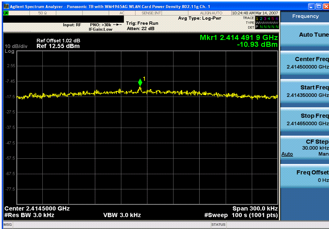
Plot 6-7. Power Spectral Density Plot (802.11g – Ch. 1)
