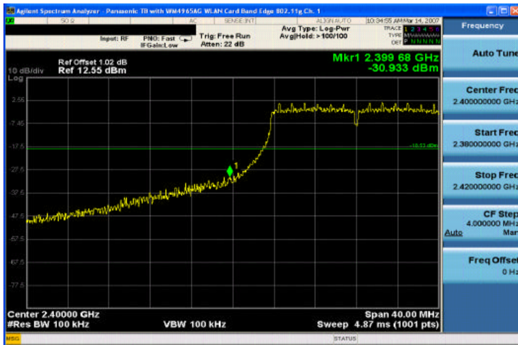
Plot 6-13. Band Edge Plot (802.11g– Ch. 1)
