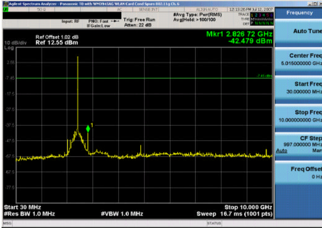
Plot 6-19. Conducted Spurious Plot (802.11g – Ch. 6)
