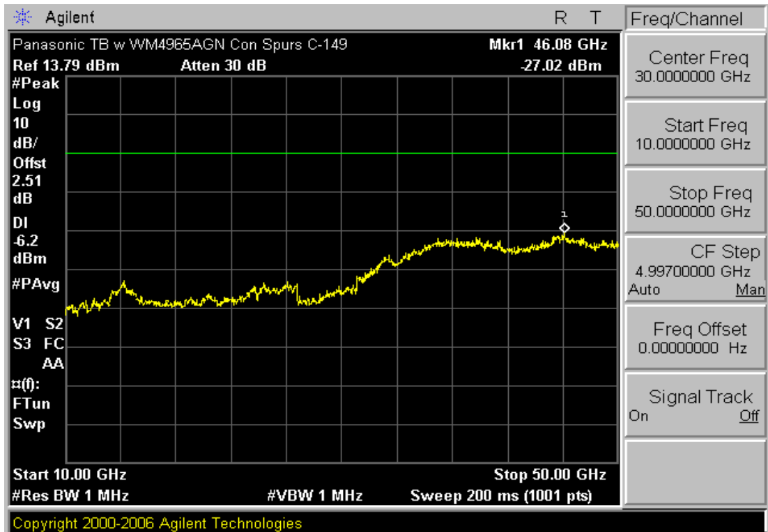
Plot 6-24. Conducted Spurious Plot (802.11a – Ch. 149)
