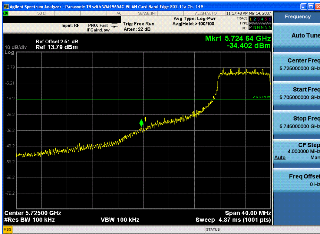
Plot 6-15. Band Edge Plot (802.11a – Ch. 149)
