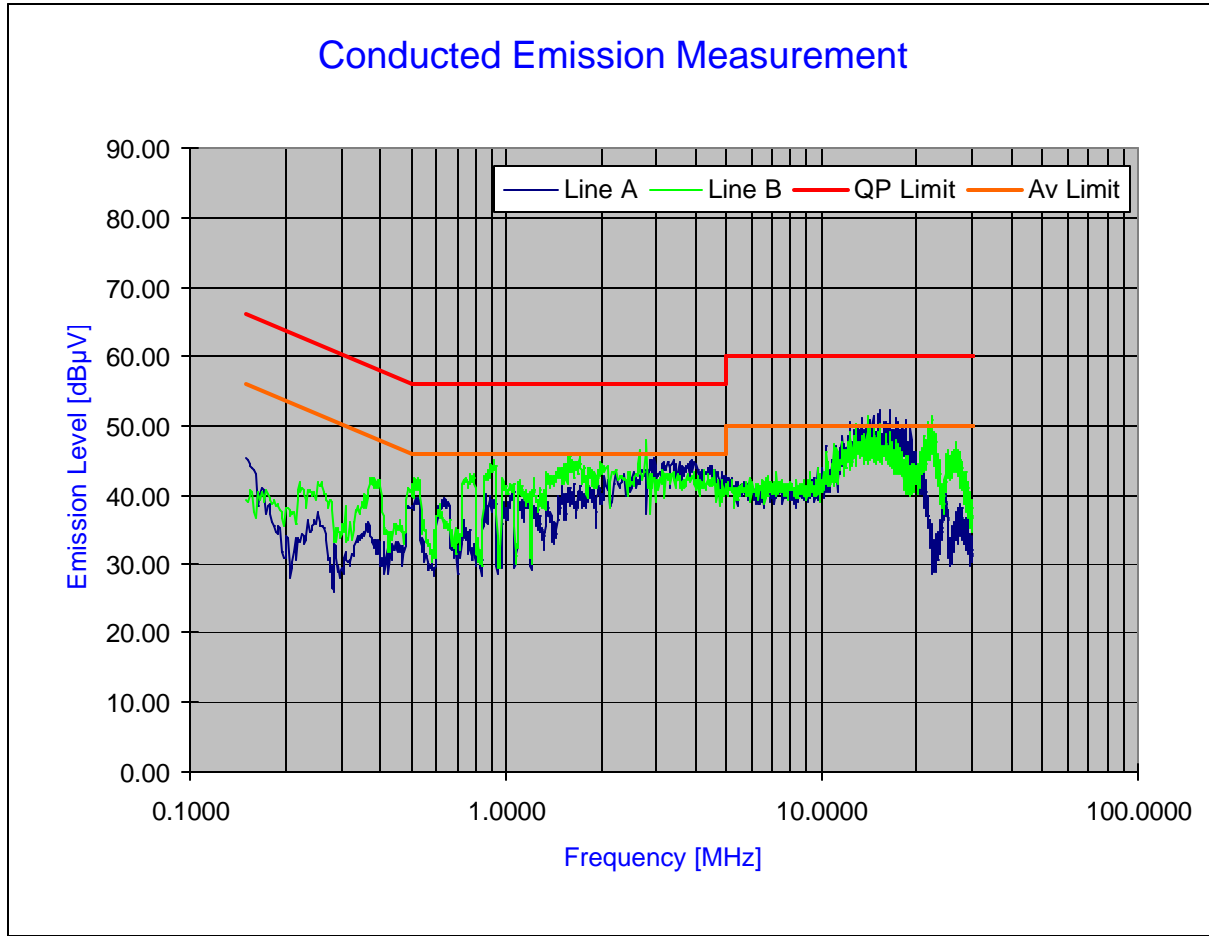
Plot 6-29. Line Conducted Plot with 802.11g
