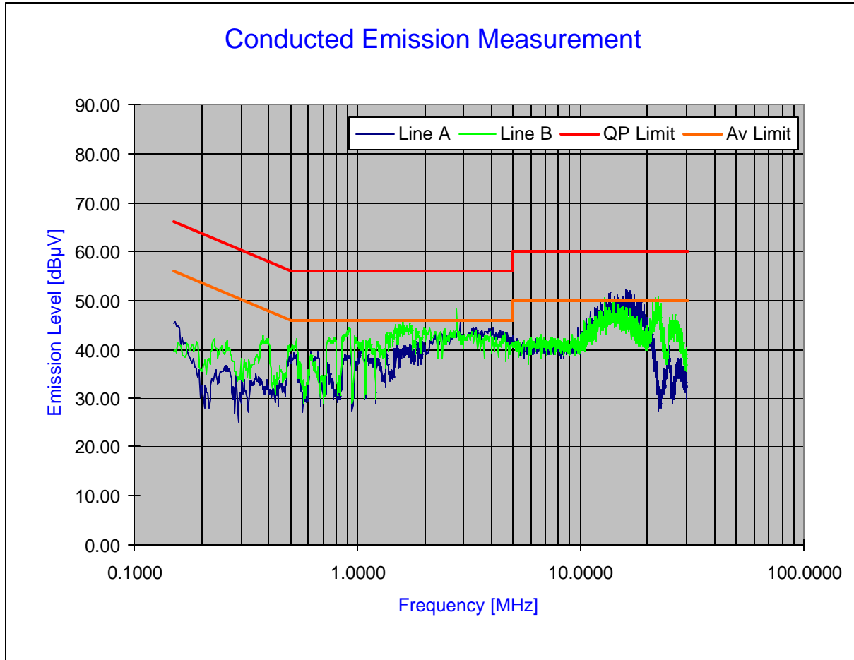
Plot 6-30. Line Conducted Plot with 802.11a
