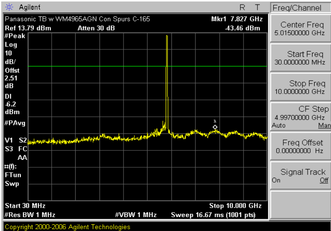
Plot 6-27. Conducted Spurious Plot (802.11a – Ch. 165)
