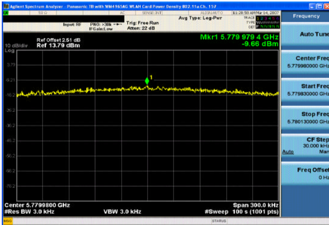
Plot 6-11. Power Spectral Density Plot (802.11a – Ch. 157)
