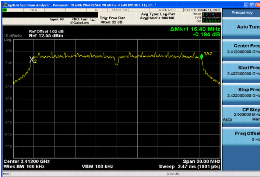
Plot 6-1. 6dB Bandwidth Plot (802.11g – Ch. 1)
