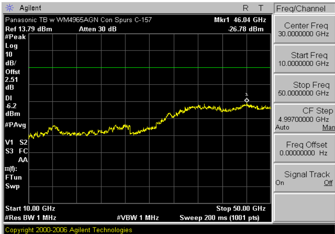
Plot 6-26. Conducted Spurious Plot (802.11a – Ch. 157)
