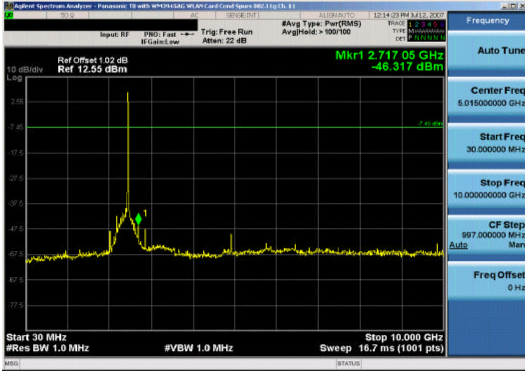
Plot 6-21. Conducted Spurious Plot (802.11g – Ch. 11)
