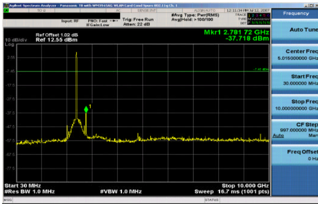
Plot 6-17. Conducted Spurious Plot (802.11g – Ch. 1)
