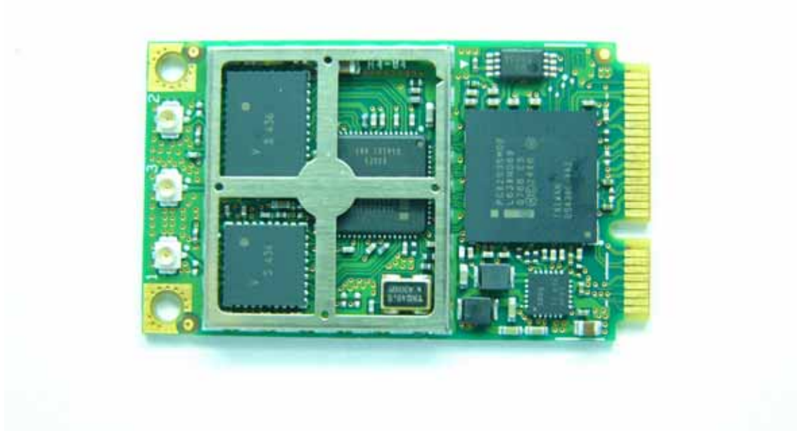
WLAN inside Top View
