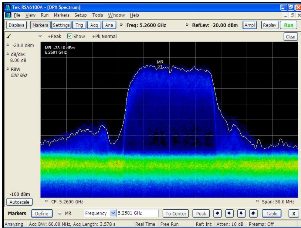
Figure 4: Real-Time Spectrum Display, WLAN Traffic (Streaming Video)
