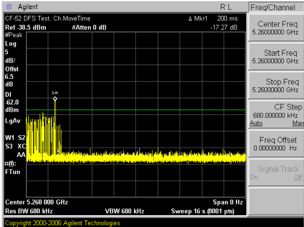
Figure 5: Channel Move Time (<10sec) (1R Marker at end of burst)
