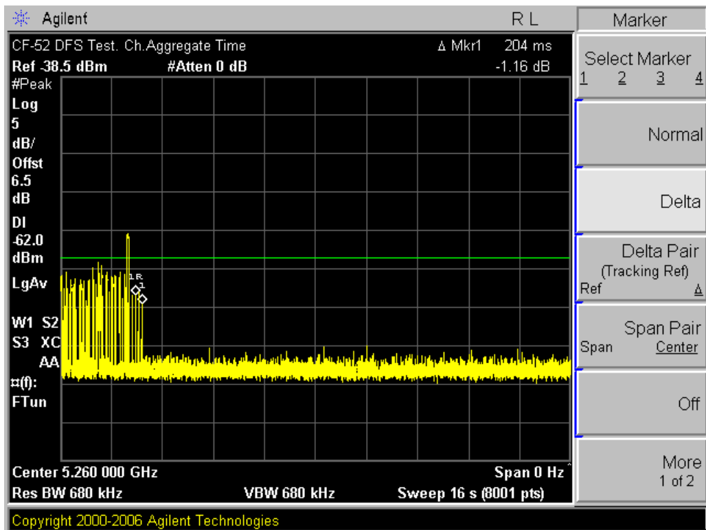
Figure 6: Channel Closing Transmission Time, (Marker 1R at 200ms after burst)
