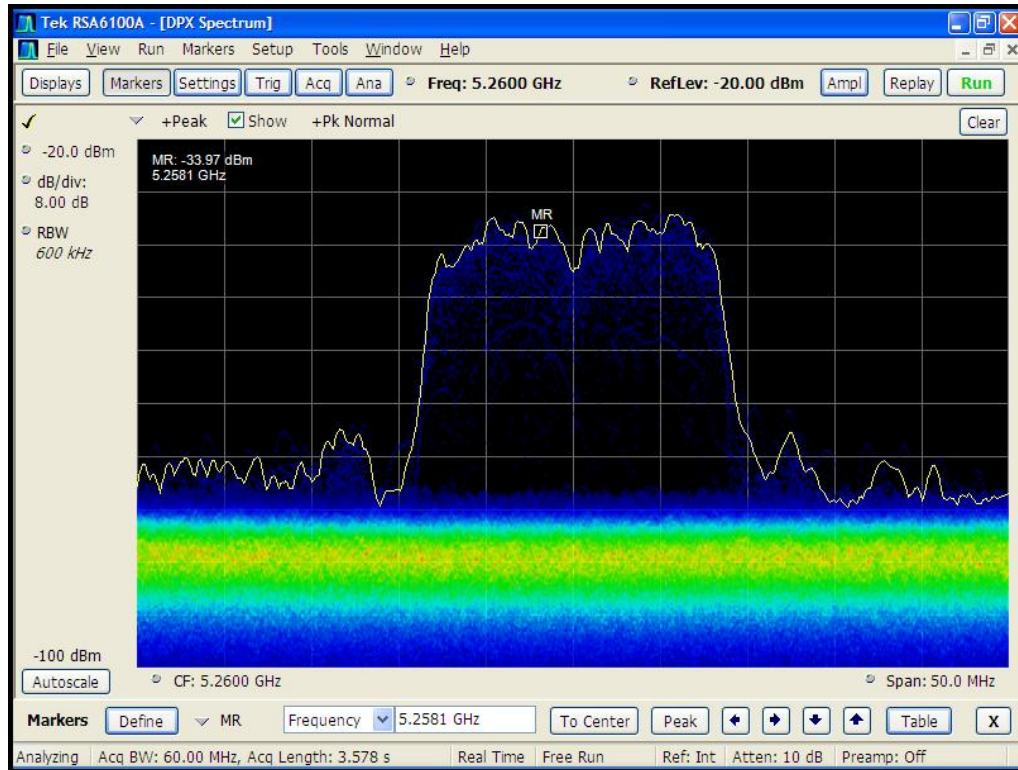
Figure 3: Real-Time Spectrum Display, No WLAN Traffic
