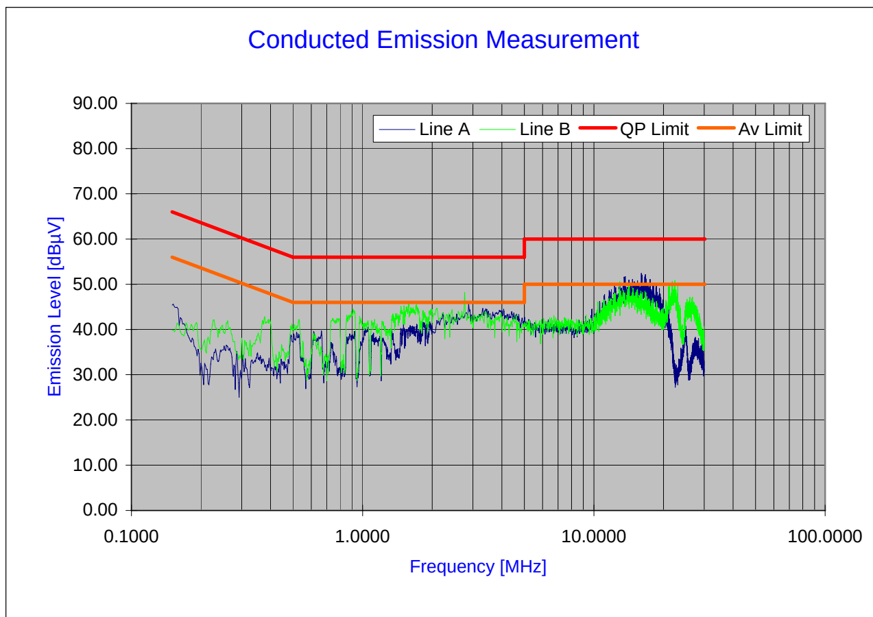
Plot 6-17. Line Conducted Plot with 802.11a
