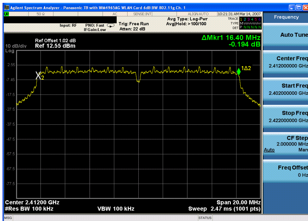
Plot 6-1. 6dB Bandwidth Plot (802.11g – Ch. 1)
