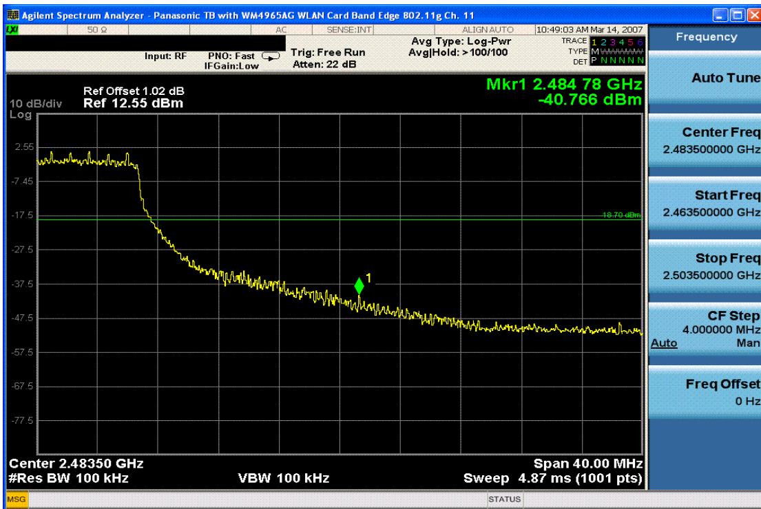
Plot 6-14. Band Edge Plot (802.11g – Ch. 11)
