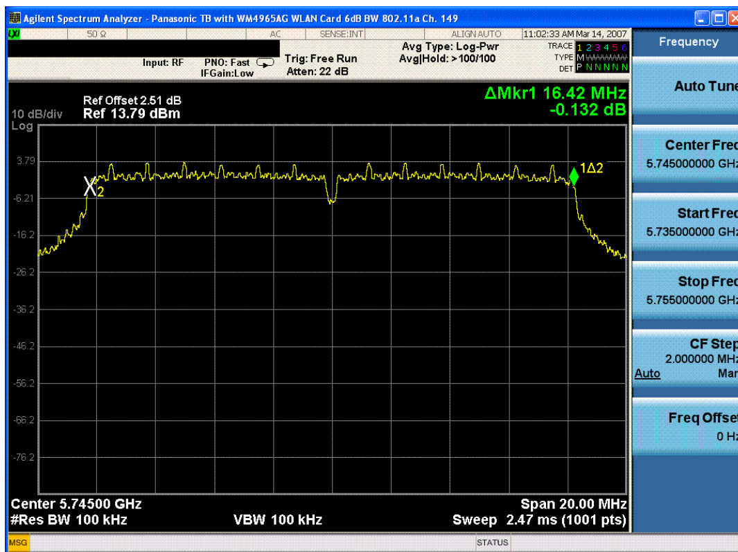
Plot 6-4. 6dB Bandwidth Plot (802.11a – Ch. 149)
