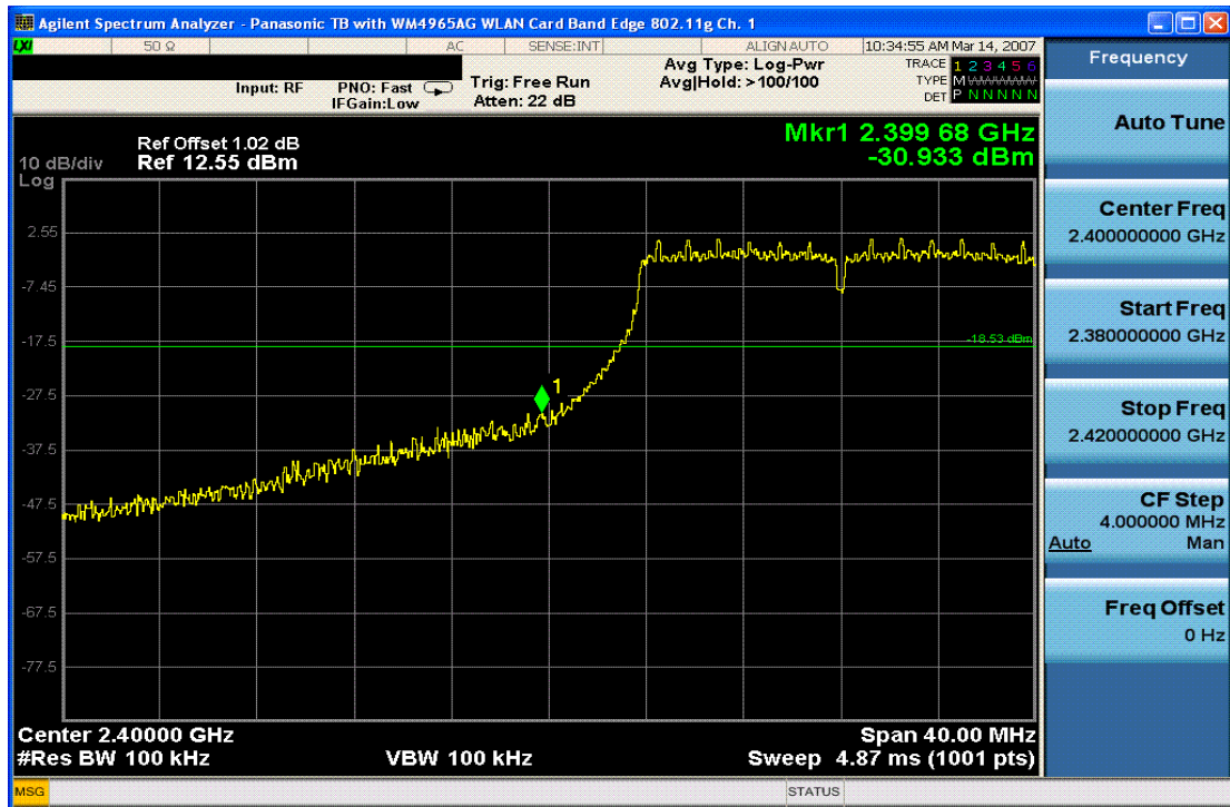
Plot 6-13. Band Edge Plot (802.11g – Ch. 1)
