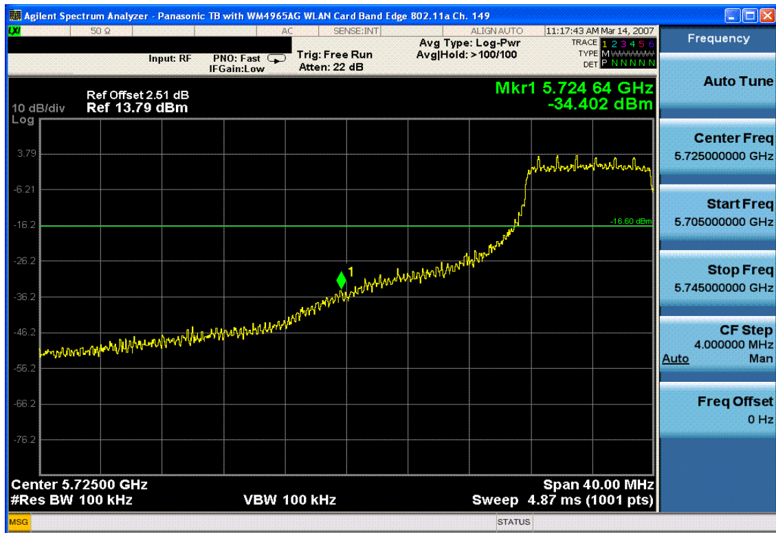
Plot 6-15. Band Edge Plot (802.11a – Ch. 149)
