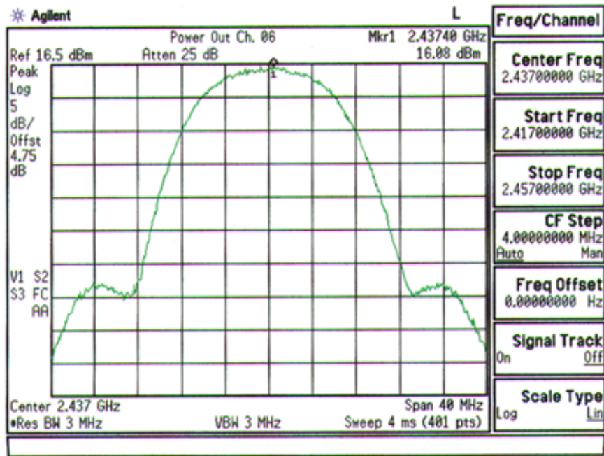
Plot A-5. Max. Output Power Plot – Ch. 06
