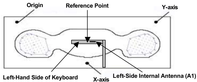
Figure 4. Phantom Reference Point & EUT Positioning Bottom Left Side of Laptop PC - Left-Side Antenna (A1)
