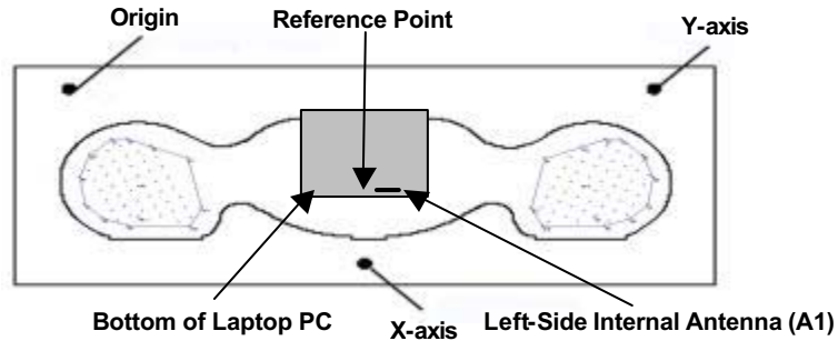
Figure 2. Phantom Reference Point & EUT Positioning Bottom Left Side of Laptop PC - Left-Side Antenna (A1)
