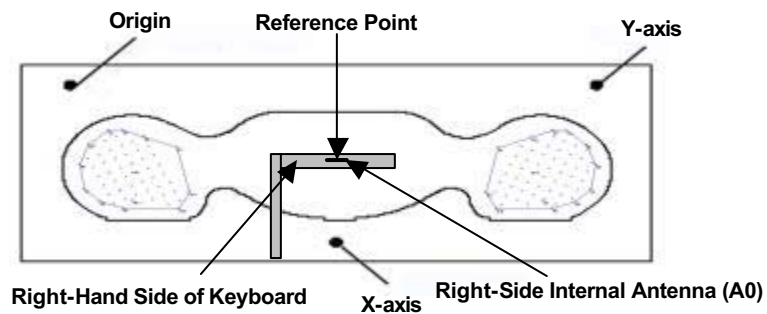
Figure 5. Phantom Reference Point & EUT Positioning Bottom Right Side of Laptop PC - Right-Side Antenna (A0)
