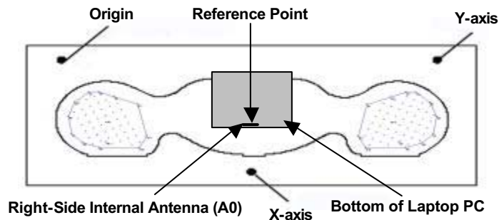
Figure 3. Phantom Reference Point & EUT Positioning Bottom Right Side of Laptop PC - Right-Side Antenna (A0)
