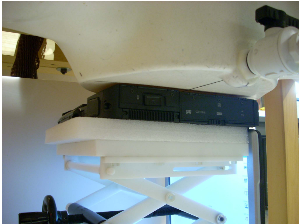
Figure 19-2 SAR Test Setup Photo 2 (Lap Position)
