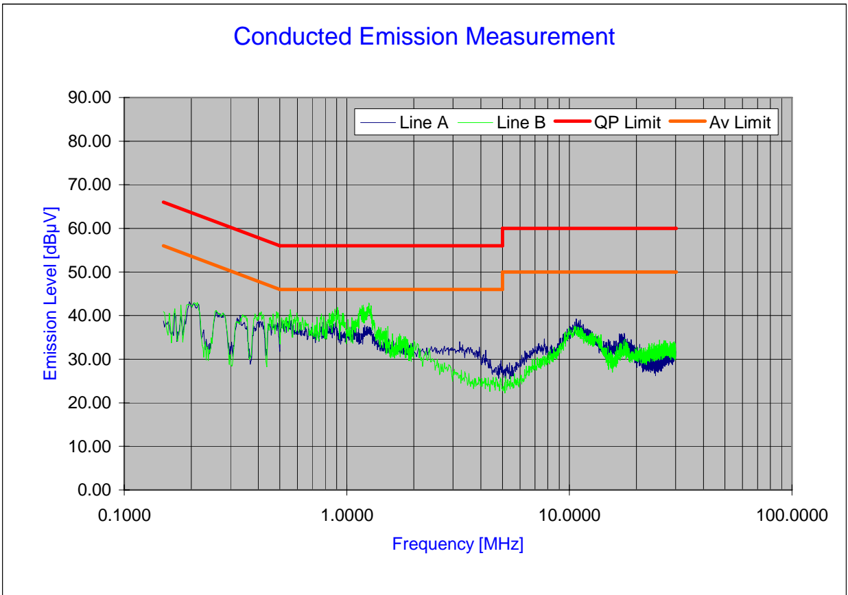
Plot 6-60. Line Conducted Plot with 802.11g
