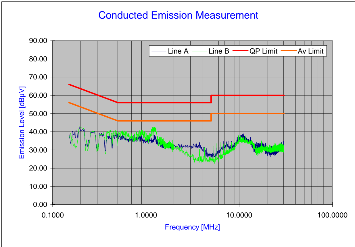
Plot 6-61. Line Conducted Plot with 802.11n
